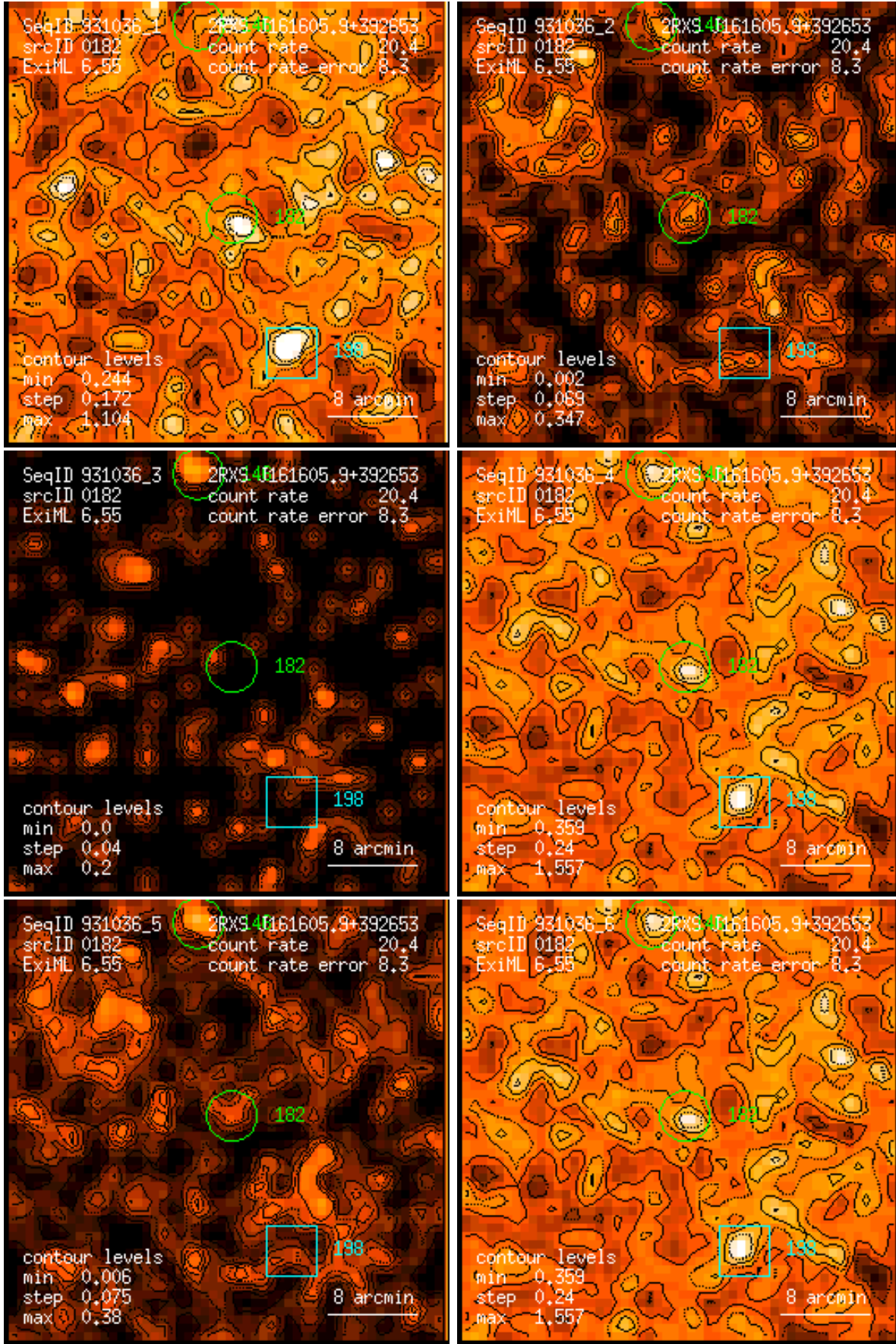
Figure 182: RASS 931036: detection 0182: band rate images, Gaussian filter: (1) PSPC channels 11 – 41, (2) 52 – 90, (3) 91 – 201, (4) 11 – 235, (5) 52 – 201, (6) 11 – 201. Broad band rates in counts/ks. Band rate contour levels in counts/ks/arcmin 2 .
