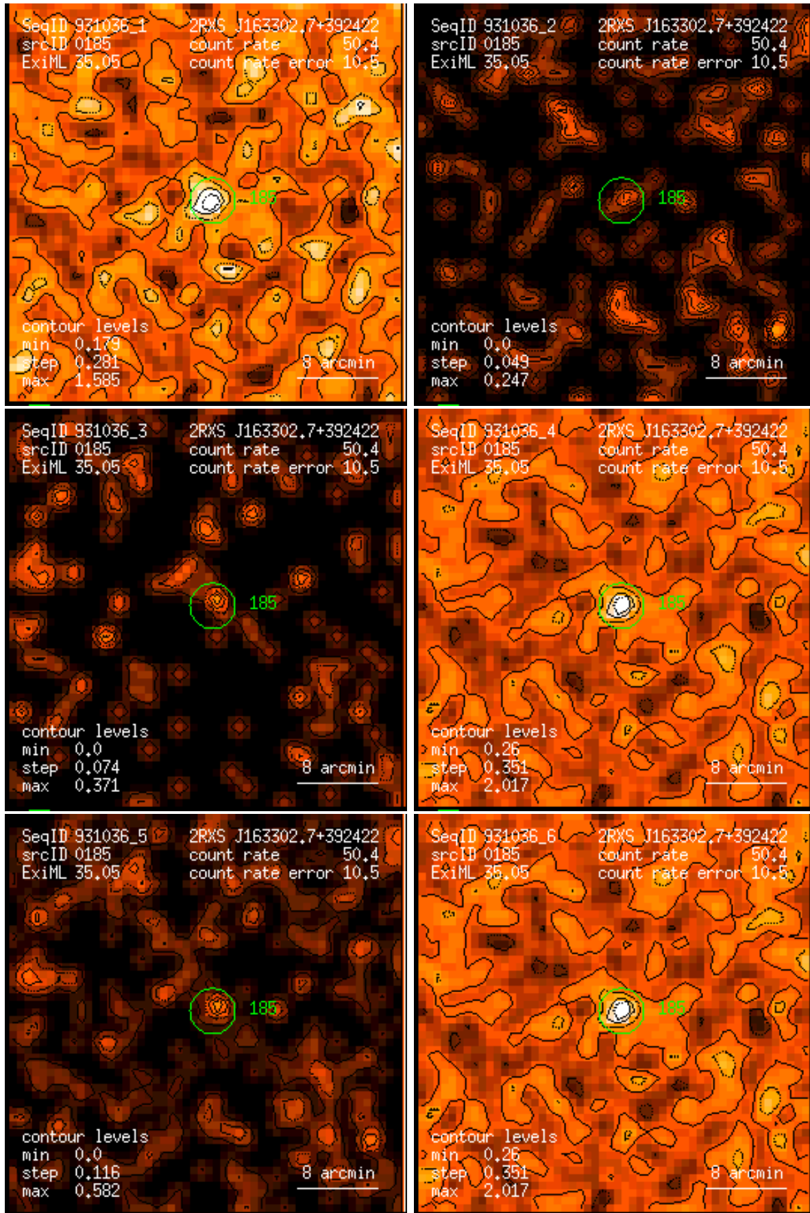
Figure 185: RASS 931036: detection 0185: band rate images, Gaussian filter: (1) PSPC channels 11 – 41, (2) 52 – 90, (3) 91 – 201, (4) 11 – 235, (5) 52 – 201, (6) 11 – 201. Broad band rates in counts/ks. Band rate contour levels in counts/ks/arcmin 2 .
