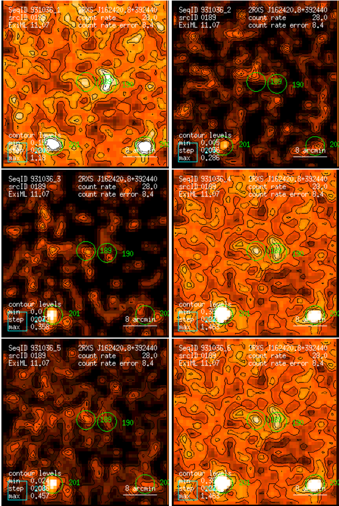
Figure 189: RASS 931036: detection 0189: band rate images, Gaussian filter: (1) PSPC channels 11 – 41, (2) 52 – 90, (3) 91 – 201, (4) 11 – 235, (5) 52 – 201, (6) 11 – 201. Broad band rates in counts/ks. Band rate contour levels in counts/ks/arcmin 2 .
