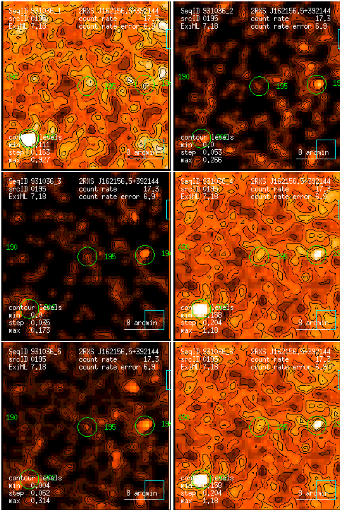
Figure 195: RASS 931036: detection 0195: band rate images, Gaussian filter: (1) PSPC channels 11 – 41, (2) 52 – 90, (3) 91 – 201, (4) 11 – 235, (5) 52 – 201, (6) 11 – 201. Broad band rates in counts/ks. Band rate contour levels in counts/ks/arcmin 2 .
