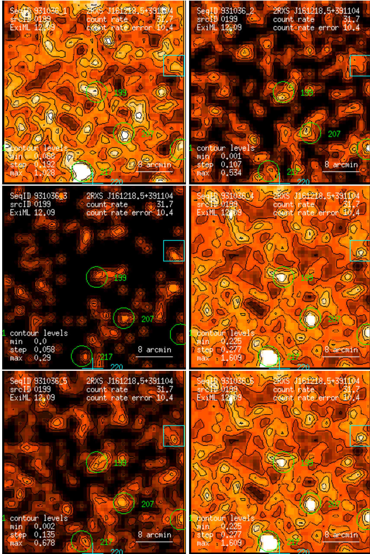
Figure 199: RASS 931036: detection 0199: band rate images, Gaussian filter: (1) PSPC channels 11 – 41, (2) 52 – 90, (3) 91 – 201, (4) 11 – 235, (5) 52 – 201, (6) 11 – 201. Broad band rates in counts/ks. Band rate contour levels in counts/ks/arcmin 2 .
