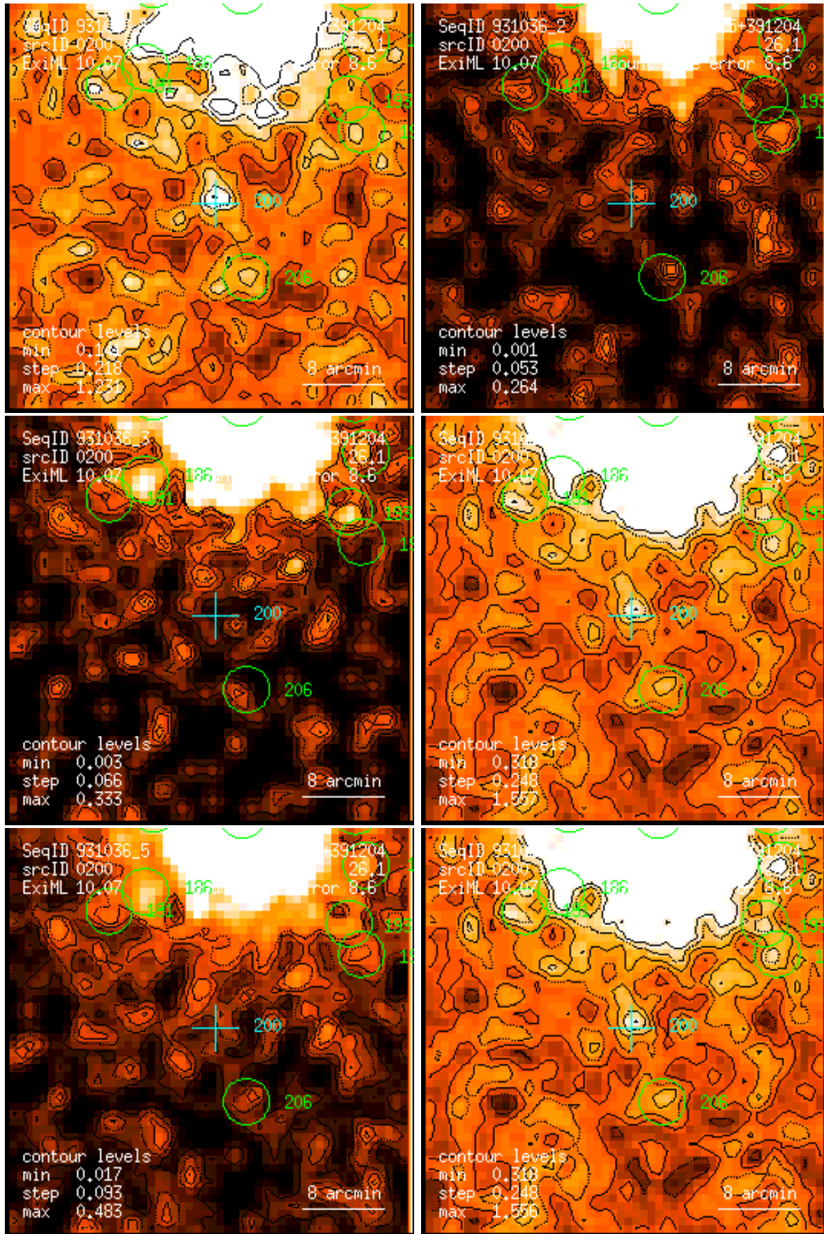
Figure 200: RASS 931036: detection 0200: band rate images, Gaussian filter: (1) PSPC channels 11 – 41, (2) 52 – 90, (3) 91 – 201, (4) 11 – 235, (5) 52 – 201, (6) 11 – 201. Broad band rates in counts/ks. Band rate contour levels in counts/ks/arcmin 2 .
