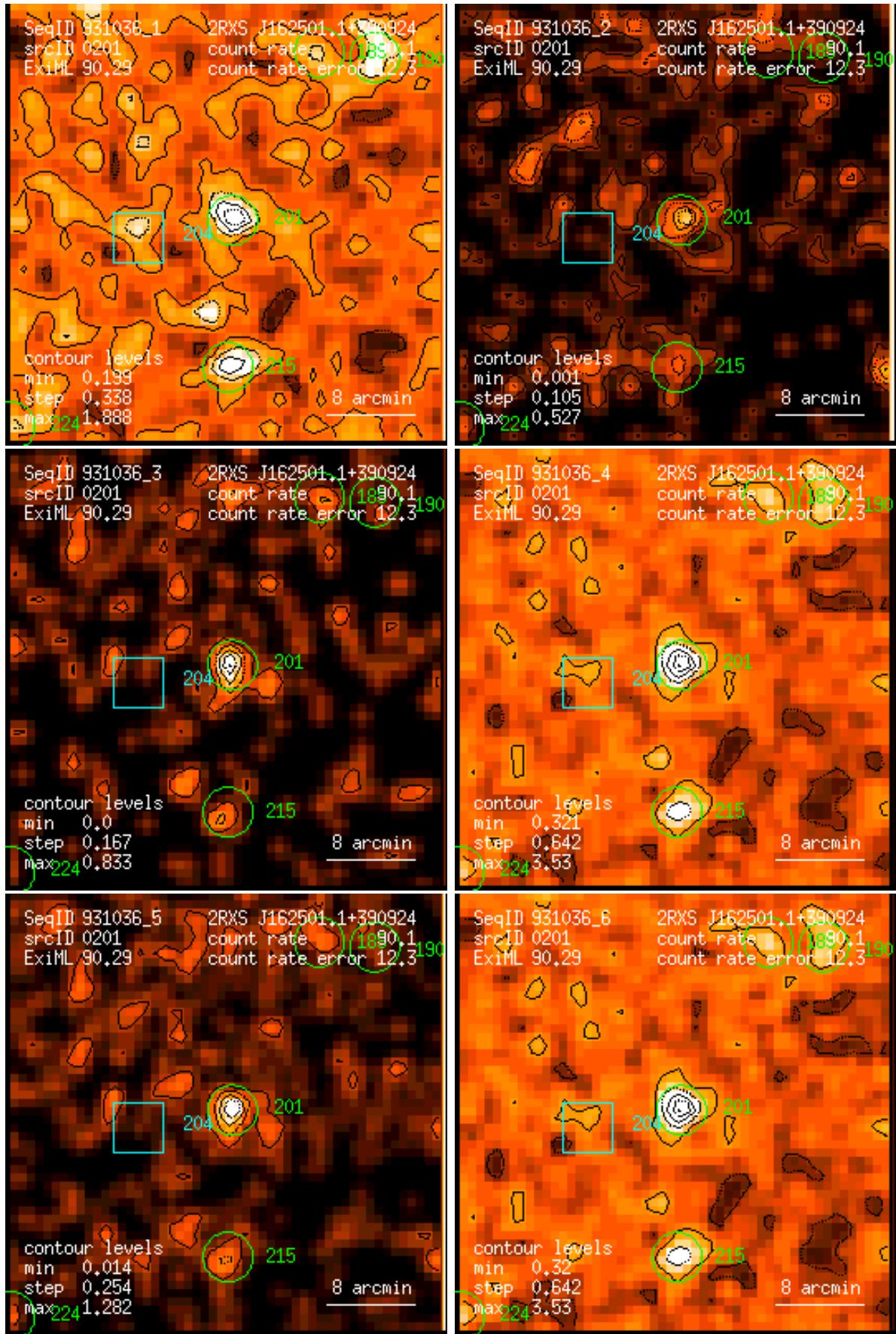
Figure 201: RASS 931036: detection 0201: band rate images, Gaussian filter: (1) PSPC channels 11 – 41, (2) 52 – 90, (3) 91 – 201, (4) 11 – 235, (5) 52 – 201, (6) 11 – 201. Broad band rates in counts/ks. Band rate contour levels in counts/ks/arcmin 2 .
