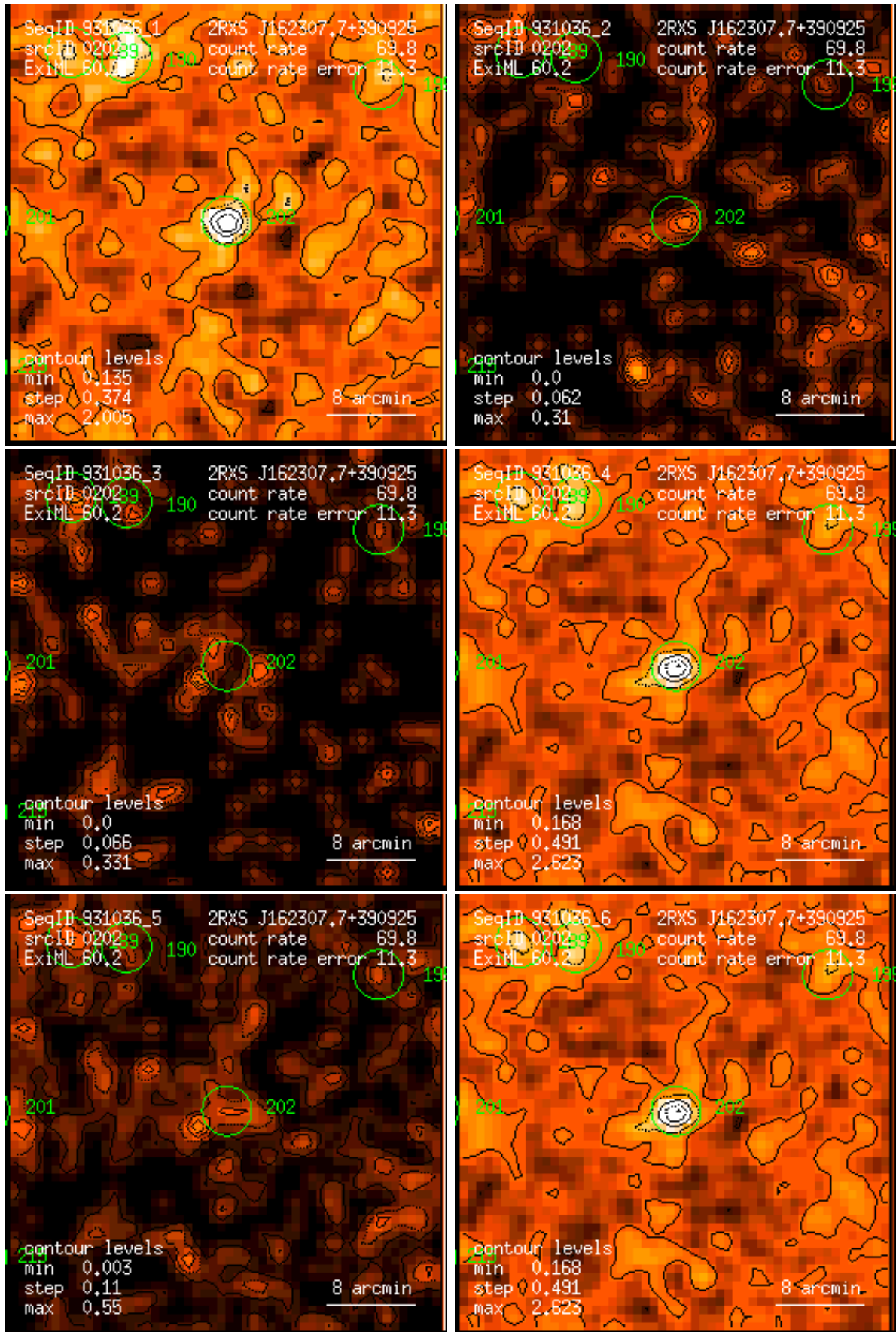
Figure 202: RASS 931036: detection 0202: band rate images, Gaussian filter: (1) PSPC channels 11 – 41, (2) 52 – 90, (3) 91 – 201, (4) 11 – 235, (5) 52 – 201, (6) 11 – 201. Broad band rates in counts/ks. Band rate contour levels in counts/ks/arcmin 2 .
