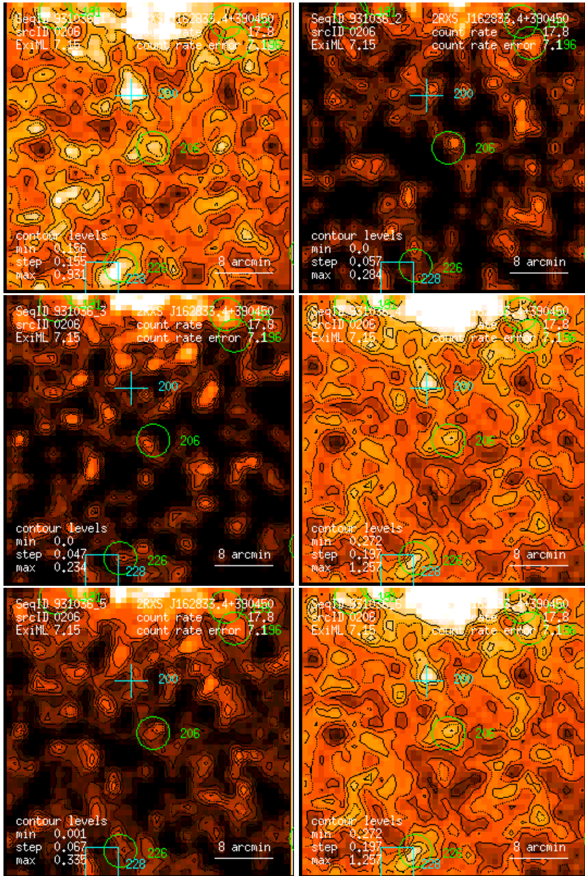
Figure 206: RASS 931036: detection 0206: band rate images, Gaussian filter: (1) PSPC channels 11 – 41, (2) 52 – 90, (3) 91 – 201, (4) 11 – 235, (5) 52 – 201, (6) 11 – 201. Broad band rates in counts/ks. Band rate contour levels in counts/ks/arcmin 2 .
