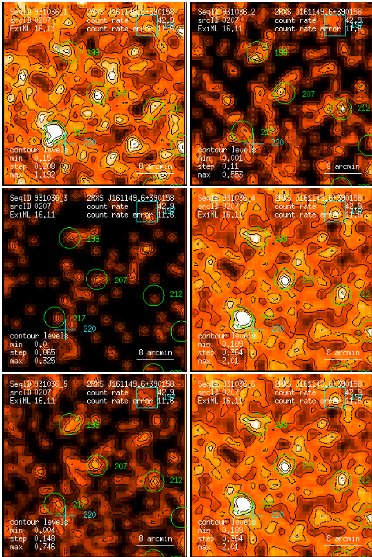
Figure 207: RASS 931036: detection 0207: band rate images, Gaussian filter: (1) PSPC channels 11 – 41, (2) 52 – 90, (3) 91 – 201, (4) 11 – 235, (5) 52 – 201, (6) 11 – 201. Broad band rates in counts/ks. Band rate contour levels in counts/ks/arcmin 2 .
