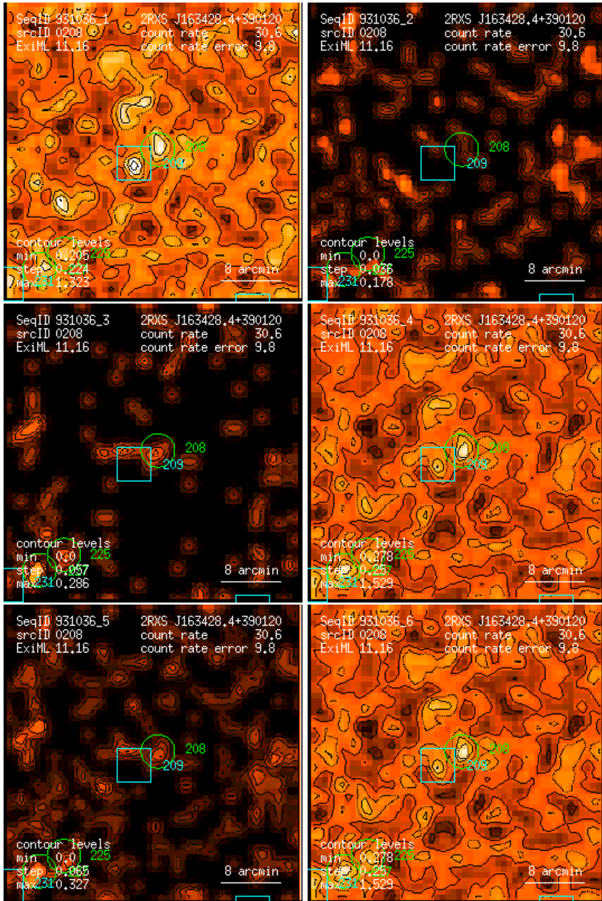
Figure 208: RASS 931036: detection 0208: band rate images, Gaussian filter: (1) PSPC channels 11 – 41, (2) 52 – 90, (3) 91 – 201, (4) 11 – 235, (5) 52 – 201, (6) 11 – 201. Broad band rates in counts/ks. Band rate contour levels in counts/ks/arcmin 2 .
