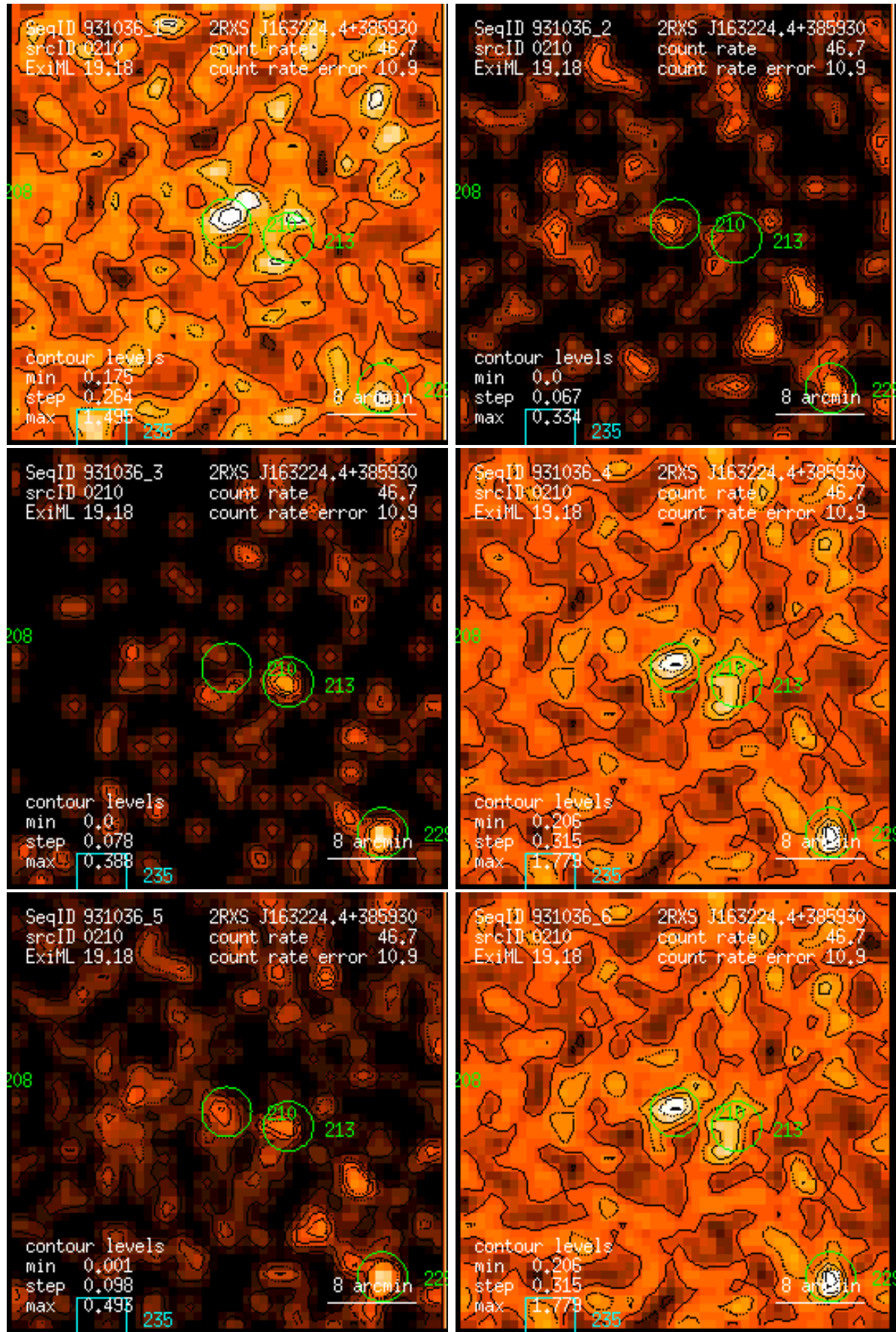
Figure 210: RASS 931036: detection 0210: band rate images, Gaussian filter: (1) PSPC channels 11 – 41, (2) 52 – 90, (3) 91 – 201, (4) 11 – 235, (5) 52 – 201, (6) 11 – 201. Broad band rates in counts/ks. Band rate contour levels in counts/ks/arcmin 2 .
