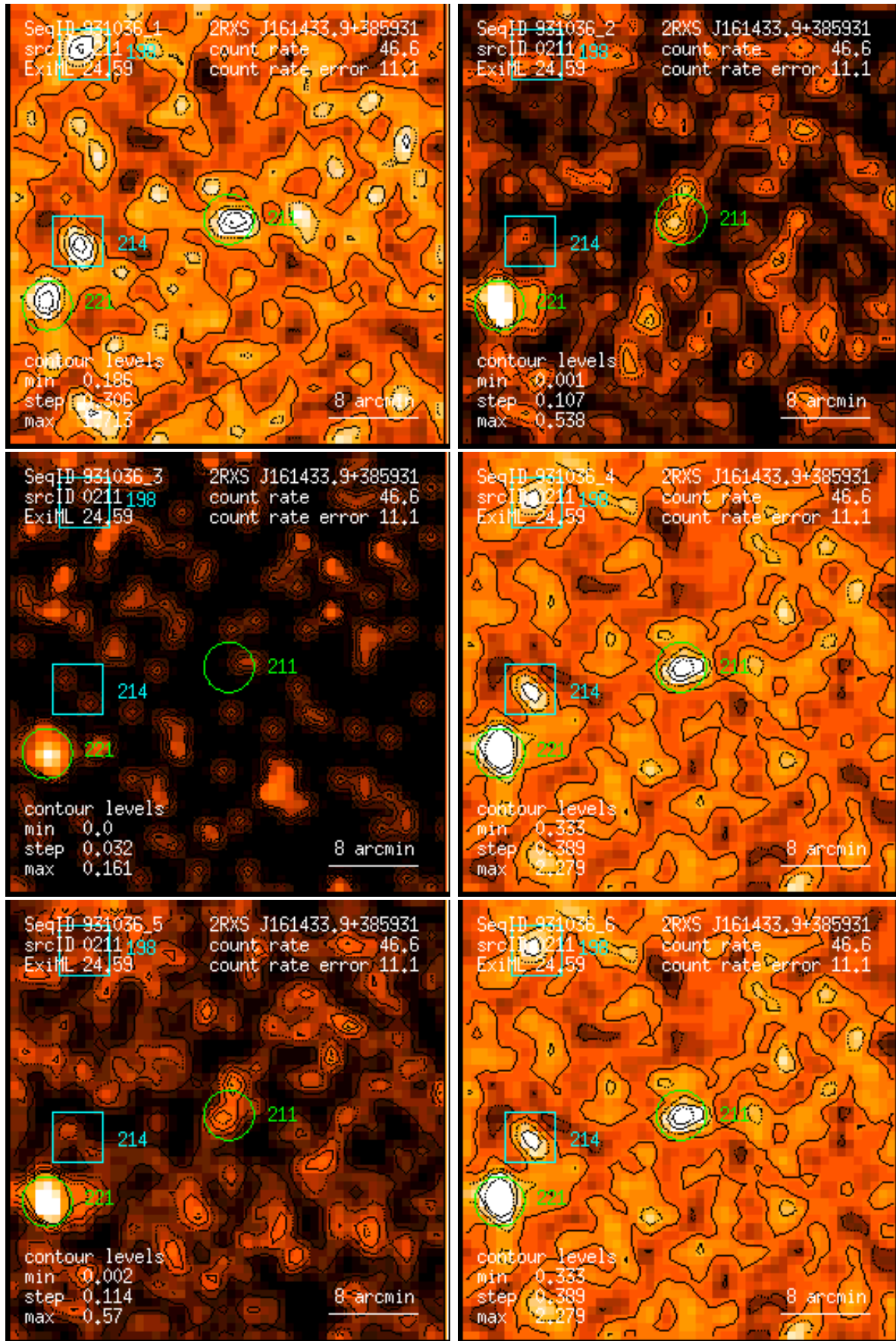
Figure 211: RASS 931036: detection 0211: band rate images, Gaussian filter: (1) PSPC channels 11 – 41, (2) 52 – 90, (3) 91 – 201, (4) 11 – 235, (5) 52 – 201, (6) 11 – 201. Broad band rates in counts/ks. Band rate contour levels in counts/ks/arcmin 2 .
