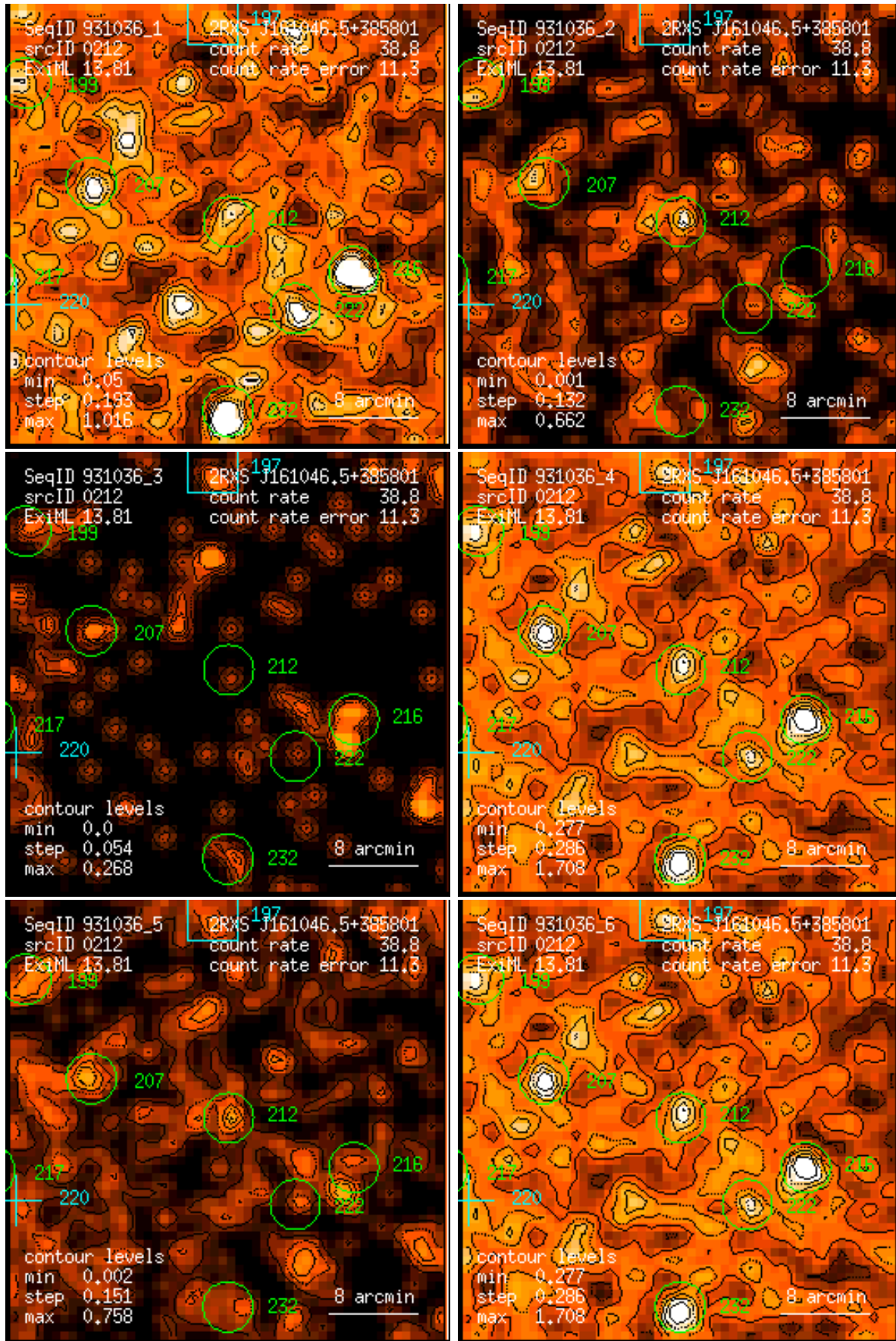
Figure 212: RASS 931036: detection 0212: band rate images, Gaussian filter: (1) PSPC channels 11 – 41, (2) 52 – 90, (3) 91 – 201, (4) 11 – 235, (5) 52 – 201, (6) 11 – 201. Broad band rates in counts/ks. Band rate contour levels in counts/ks/arcmin 2 .
