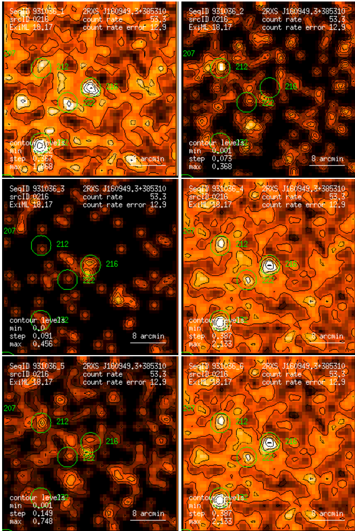
Figure 216: RASS 931036: detection 0216: band rate images, Gaussian filter: (1) PSPC channels 11 – 41, (2) 52 – 90, (3) 91 – 201, (4) 11 – 235, (5) 52 – 201, (6) 11 – 201. Broad band rates in counts/ks. Band rate contour levels in counts/ks/arcmin 2 .
