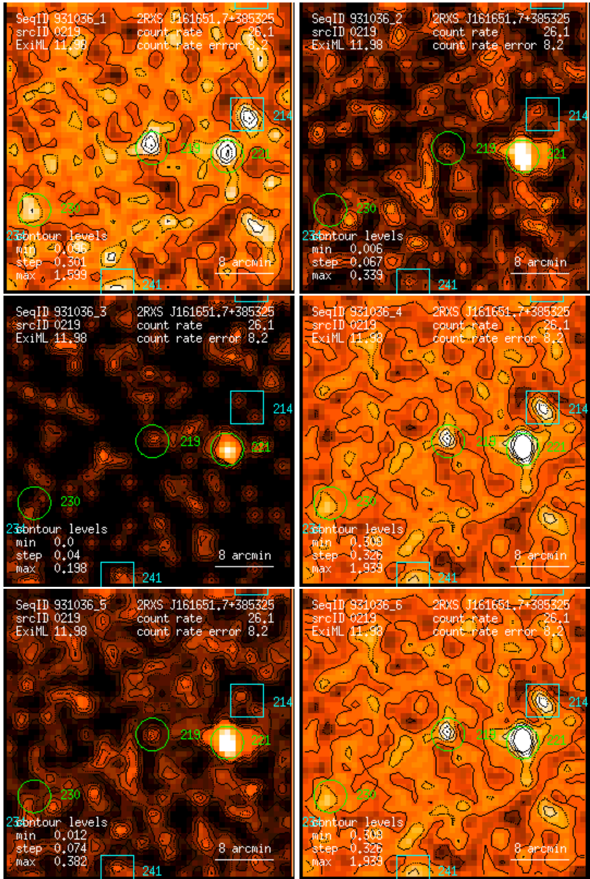
Figure 219: RASS 931036: detection 0219: band rate images, Gaussian filter: (1) PSPC channels 11 – 41, (2) 52 – 90, (3) 91 – 201, (4) 11 – 235, (5) 52 – 201, (6) 11 – 201. Broad band rates in counts/ks. Band rate contour levels in counts/ks/arcmin 2 .
