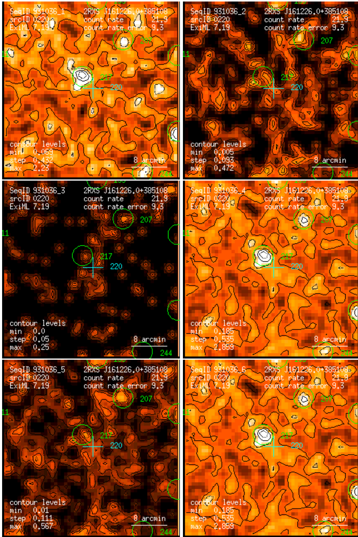
Figure 220: RASS 931036: detection 0220: band rate images, Gaussian filter: (1) PSPC channels 11 – 41, (2) 52 – 90, (3) 91 – 201, (4) 11 – 235, (5) 52 – 201, (6) 11 – 201. Broad band rates in counts/ks. Band rate contour levels in counts/ks/arcmin 2 .
