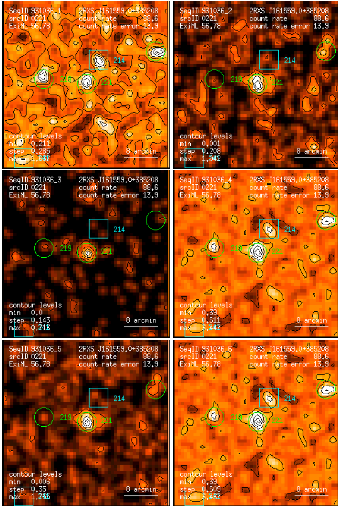
Figure 221: RASS 931036: detection 0221: band rate images, Gaussian filter: (1) PSPC channels 11 – 41, (2) 52 – 90, (3) 91 – 201, (4) 11 – 235, (5) 52 – 201, (6) 11 – 201. Broad band rates in counts/ks. Band rate contour levels in counts/ks/arcmin 2 .
