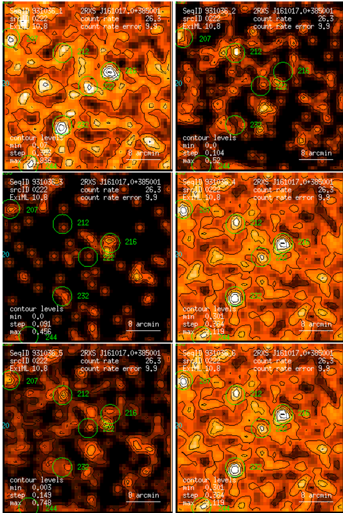
Figure 222: RASS 931036: detection 0222: band rate images, Gaussian filter: (1) PSPC channels 11 – 41, (2) 52 – 90, (3) 91 – 201, (4) 11 – 235, (5) 52 – 201, (6) 11 – 201. Broad band rates in counts/ks. Band rate contour levels in counts/ks/arcmin 2 .
