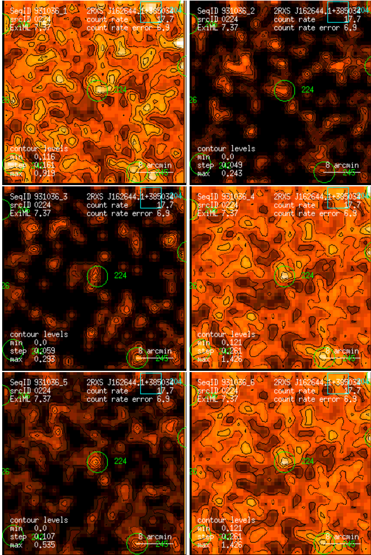
Figure 224: RASS 931036: detection 0224: band rate images, Gaussian filter: (1) PSPC channels 11 – 41, (2) 52 – 90, (3) 91 – 201, (4) 11 – 235, (5) 52 – 201, (6) 11 – 201. Broad band rates in counts/ks. Band rate contour levels in counts/ks/arcmin 2 .
