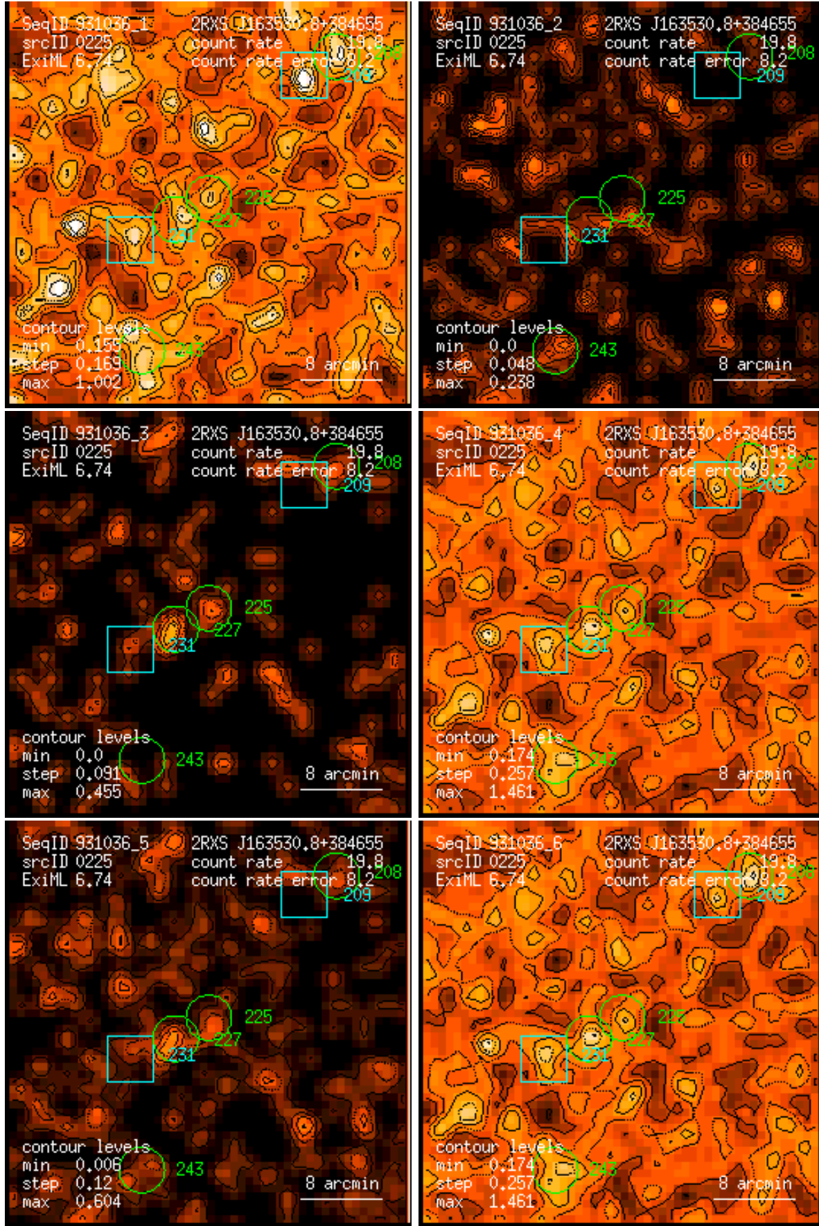
Figure 225: RASS 931036: detection 0225: band rate images, Gaussian filter: (1) PSPC channels 11 – 41, (2) 52 – 90, (3) 91 – 201, (4) 11 – 235, (5) 52 – 201, (6) 11 – 201. Broad band rates in counts/ks. Band rate contour levels in counts/ks/arcmin 2 .
