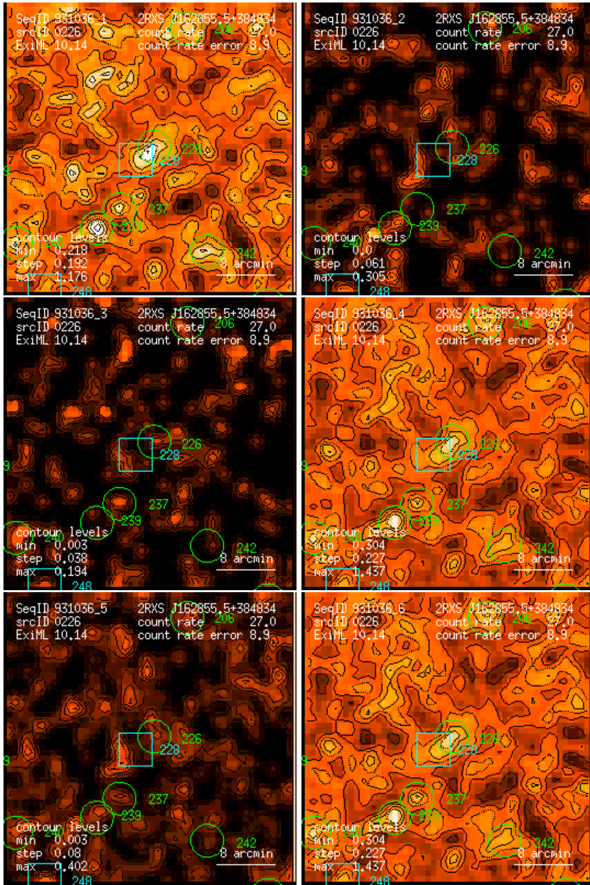
Figure 226: RASS 931036: detection 0226: band rate images, Gaussian filter: (1) PSPC channels 11 – 41, (2) 52 – 90, (3) 91 – 201, (4) 11 – 235, (5) 52 – 201, (6) 11 – 201. Broad band rates in counts/ks. Band rate contour levels in counts/ks/arcmin 2 .
