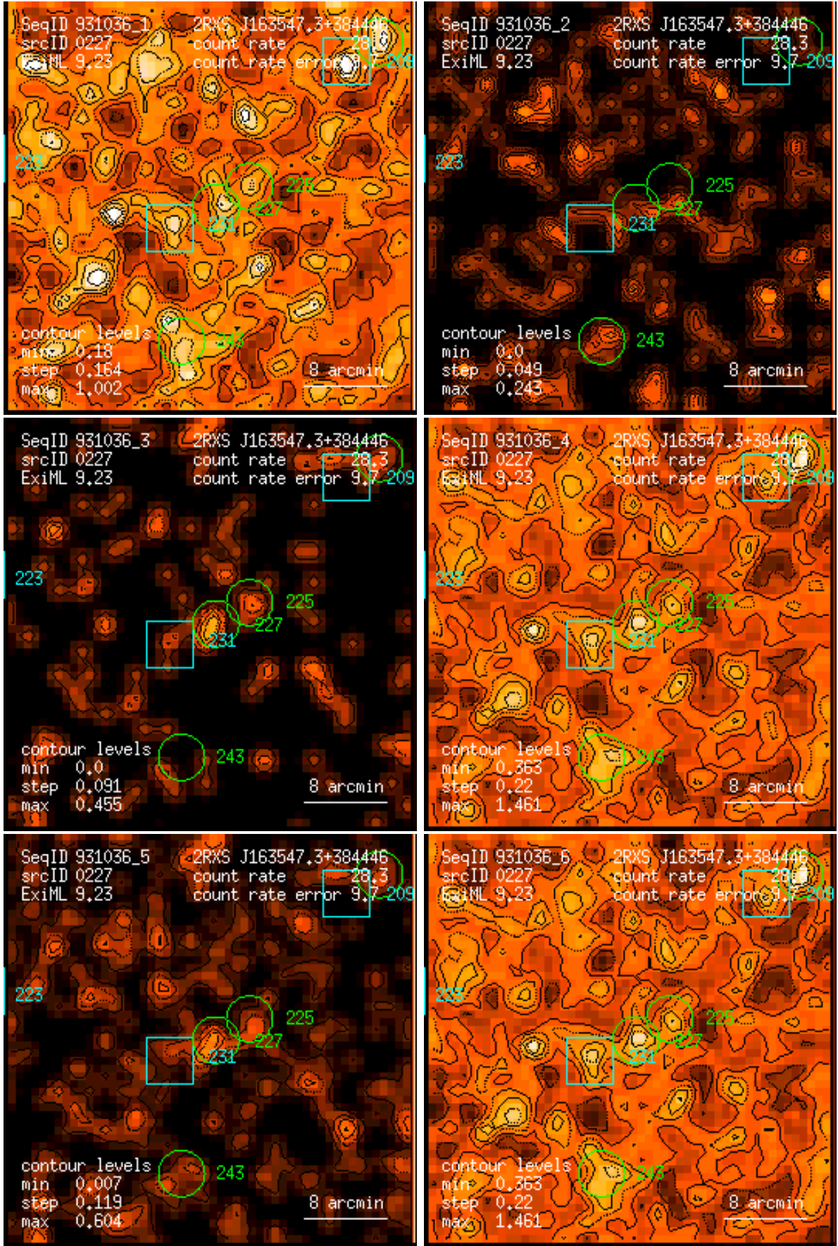
Figure 227: RASS 931036: detection 0227: band rate images, Gaussian filter: (1) PSPC channels 11 – 41, (2) 52 – 90, (3) 91 – 201, (4) 11 – 235, (5) 52 – 201, (6) 11 – 201. Broad band rates in counts/ks. Band rate contour levels in counts/ks/arcmin 2 .
