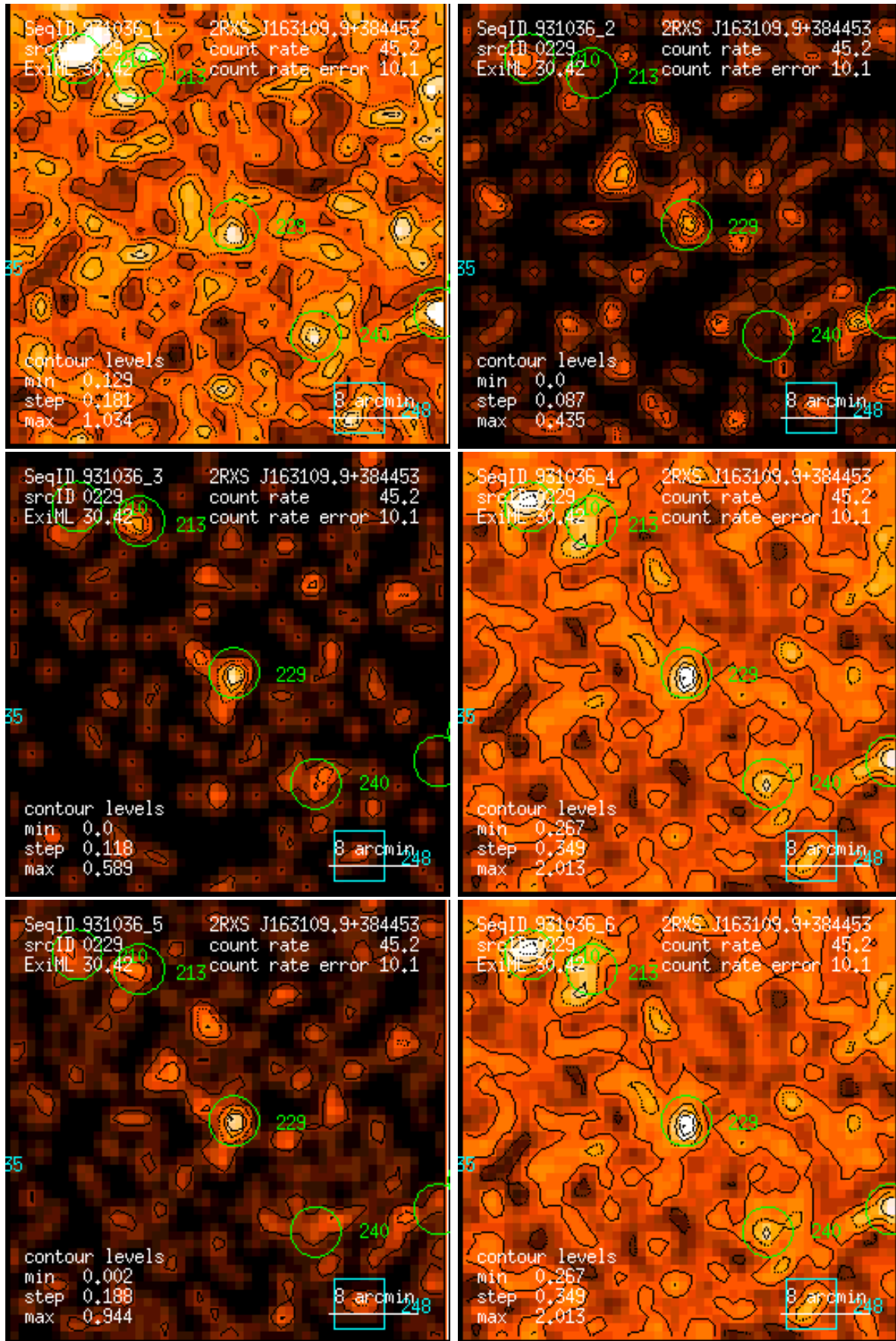
Figure 229: RASS 931036: detection 0229: band rate images, Gaussian filter: (1) PSPC channels 11 – 41, (2) 52 – 90, (3) 91 – 201, (4) 11 – 235, (5) 52 – 201, (6) 11 – 201. Broad band rates in counts/ks. Band rate contour levels in counts/ks/arcmin 2 .
