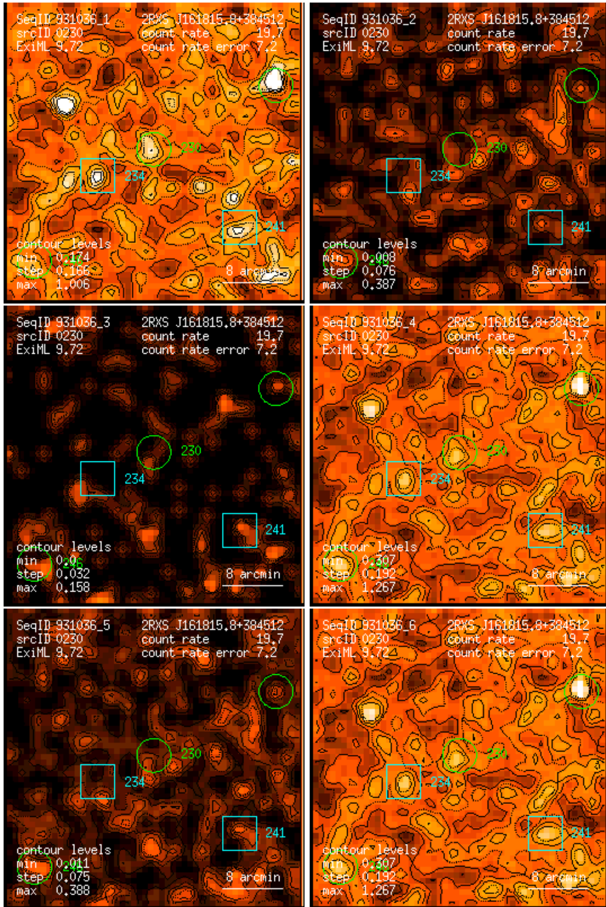
Figure 230: RASS 931036: detection 0230: band rate images, Gaussian filter: (1) PSPC channels 11 – 41, (2) 52 – 90, (3) 91 – 201, (4) 11 – 235, (5) 52 – 201, (6) 11 – 201. Broad band rates in counts/ks. Band rate contour levels in counts/ks/arcmin 2 .
