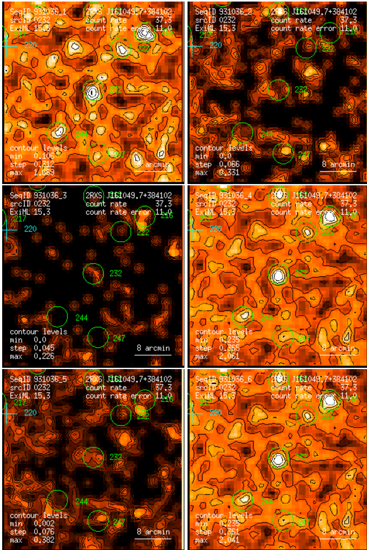
Figure 232: RASS 931036: detection 0232: band rate images, Gaussian filter: (1) PSPC channels 11 – 41, (2) 52 – 90, (3) 91 – 201, (4) 11 – 235, (5) 52 – 201, (6) 11 – 201. Broad band rates in counts/ks. Band rate contour levels in counts/ks/arcmin 2 .
