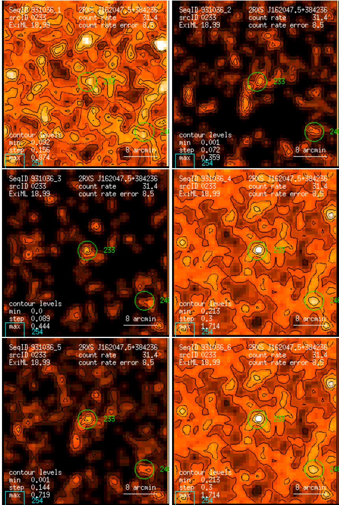
Figure 233: RASS 931036: detection 0233: band rate images, Gaussian filter: (1) PSPC channels 11 – 41, (2) 52 – 90, (3) 91 – 201, (4) 11 – 235, (5) 52 – 201, (6) 11 – 201. Broad band rates in counts/ks. Band rate contour levels in counts/ks/arcmin 2 .
