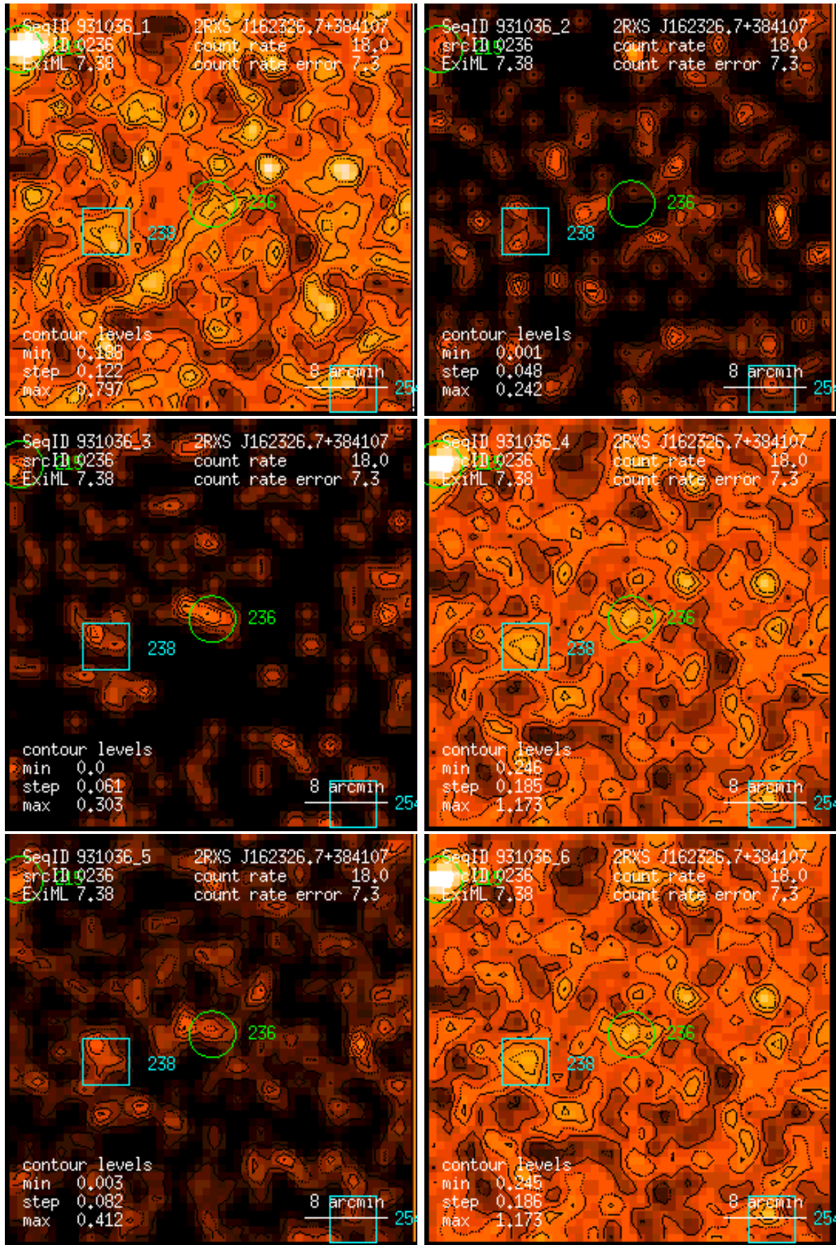
Figure 236: RASS 931036: detection 0236: band rate images, Gaussian filter: (1) PSPC channels 11 – 41, (2) 52 – 90, (3) 91 – 201, (4) 11 – 235, (5) 52 – 201, (6) 11 – 201. Broad band rates in counts/ks. Band rate contour levels in counts/ks/arcmin 2 .
