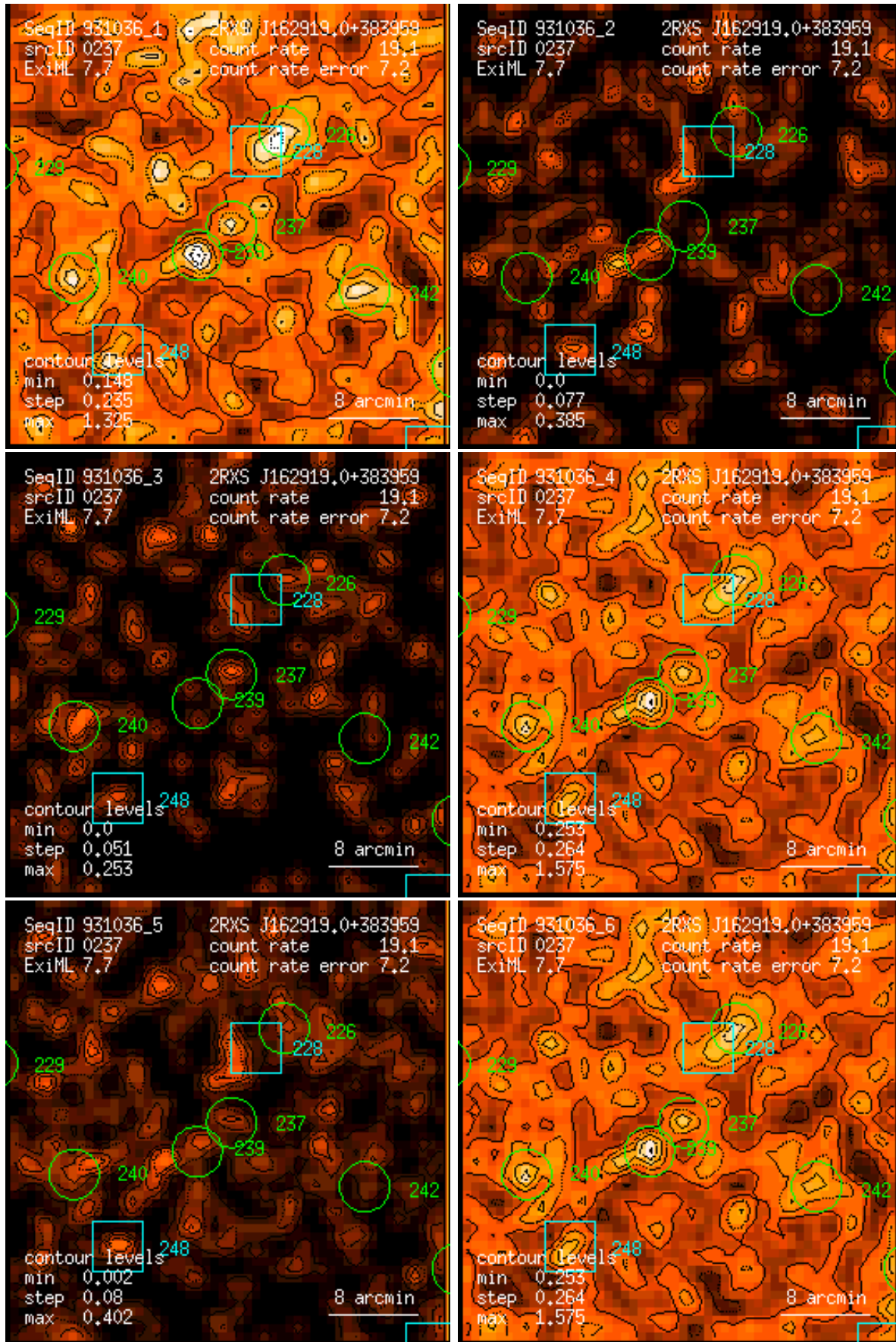
Figure 237: RASS 931036: detection 0237: band rate images, Gaussian filter: (1) PSPC channels 11 – 41, (2) 52 – 90, (3) 91 – 201, (4) 11 – 235, (5) 52 – 201, (6) 11 – 201. Broad band rates in counts/ks. Band rate contour levels in counts/ks/arcmin 2 .
