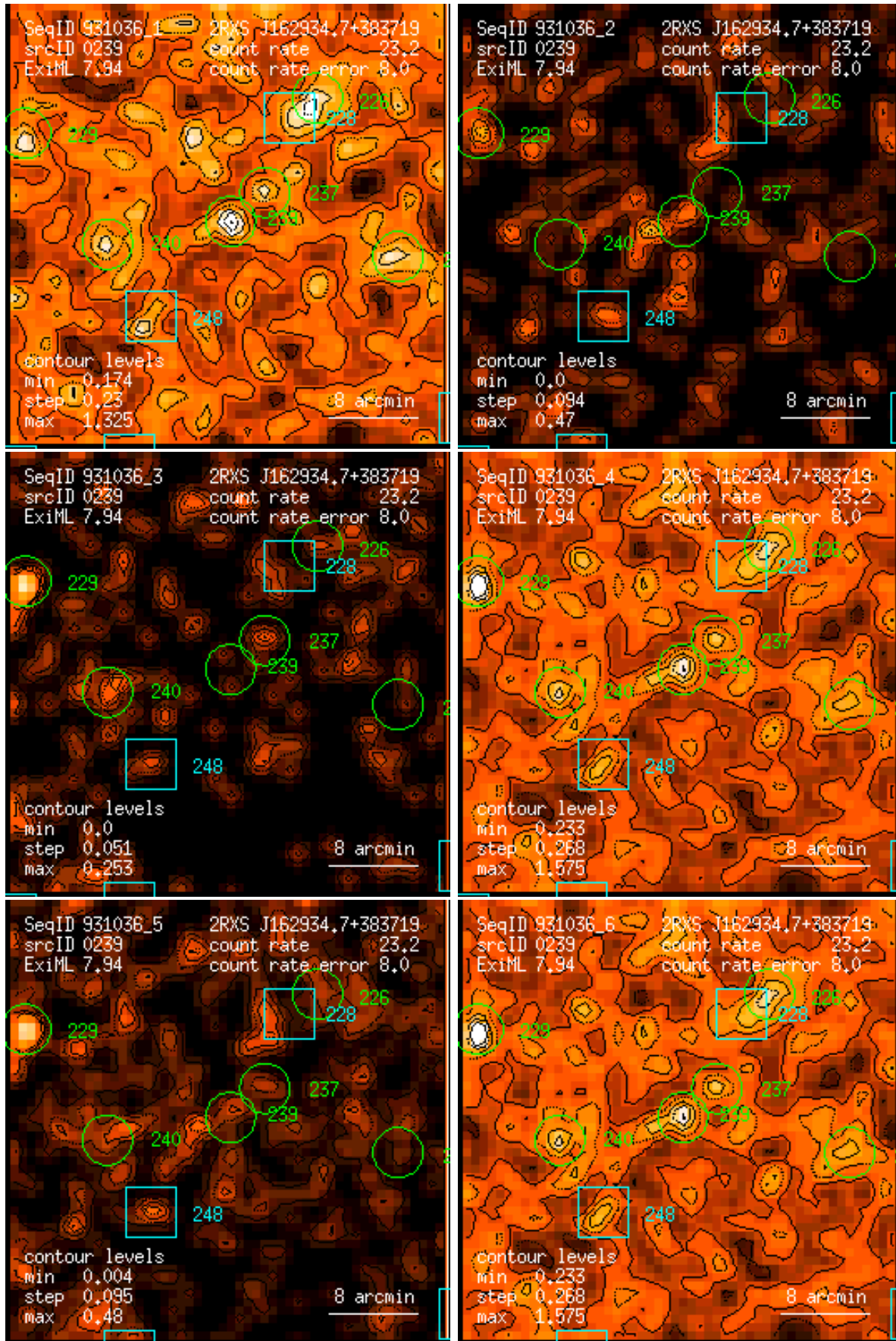
Figure 239: RASS 931036: detection 0239: band rate images, Gaussian filter: (1) PSPC channels 11 – 41, (2) 52 – 90, (3) 91 – 201, (4) 11 – 235, (5) 52 – 201, (6) 11 – 201. Broad band rates in counts/ks. Band rate contour levels in counts/ks/arcmin 2 .
