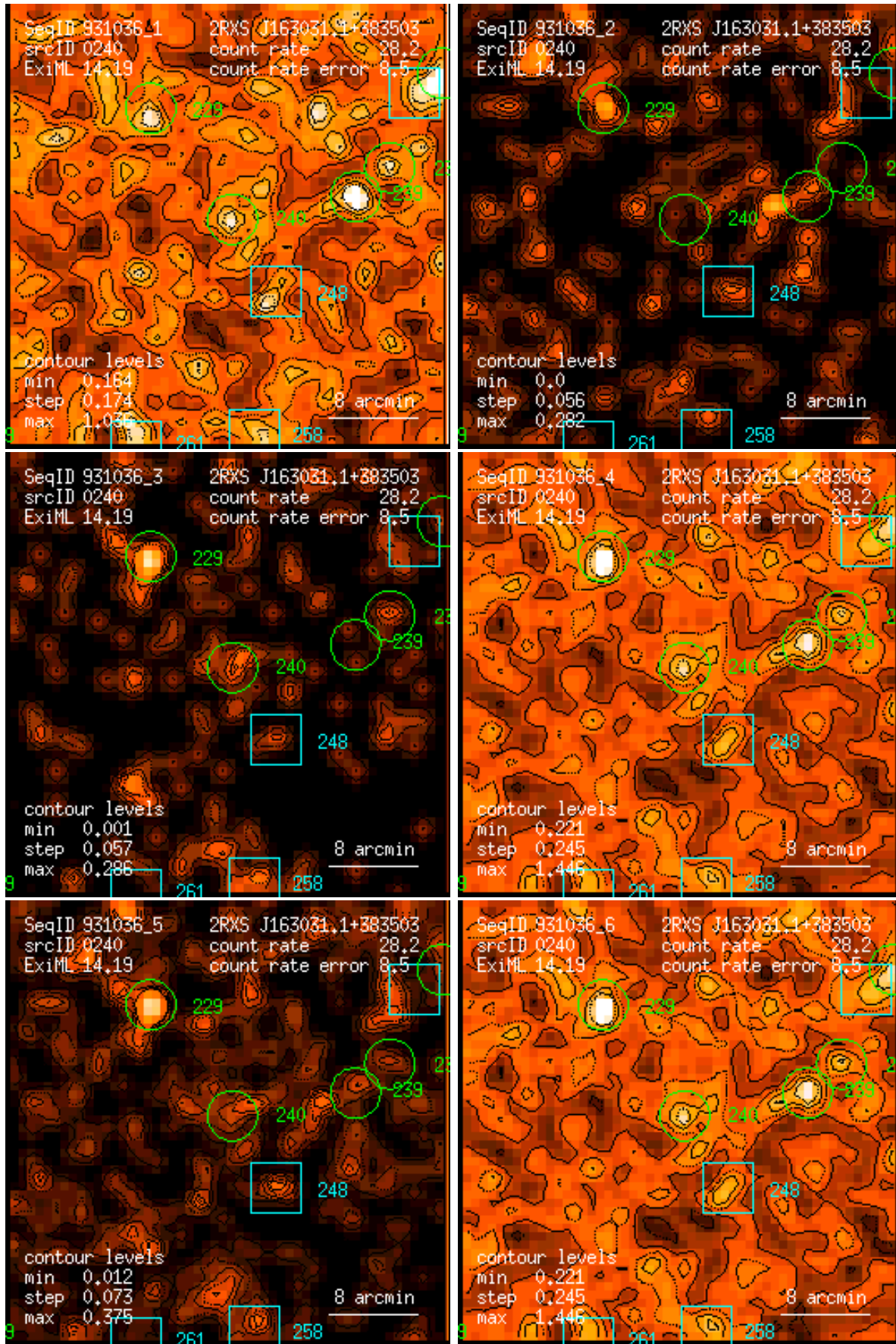
Figure 240: RASS 931036: detection 0240: band rate images, Gaussian filter: (1) PSPC channels 11 – 41, (2) 52 – 90, (3) 91 – 201, (4) 11 – 235, (5) 52 – 201, (6) 11 – 201. Broad band rates in counts/ks. Band rate contour levels in counts/ks/arcmin 2 .
