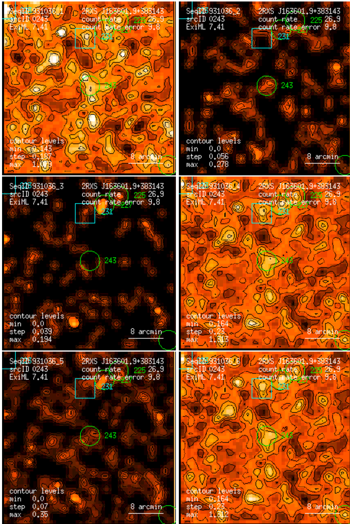
Figure 243: RASS 931036: detection 0243: band rate images, Gaussian filter: (1) PSPC channels 11 – 41, (2) 52 – 90, (3) 91 – 201, (4) 11 – 235, (5) 52 – 201, (6) 11 – 201. Broad band rates in counts/ks. Band rate contour levels in counts/ks/arcmin 2 .
