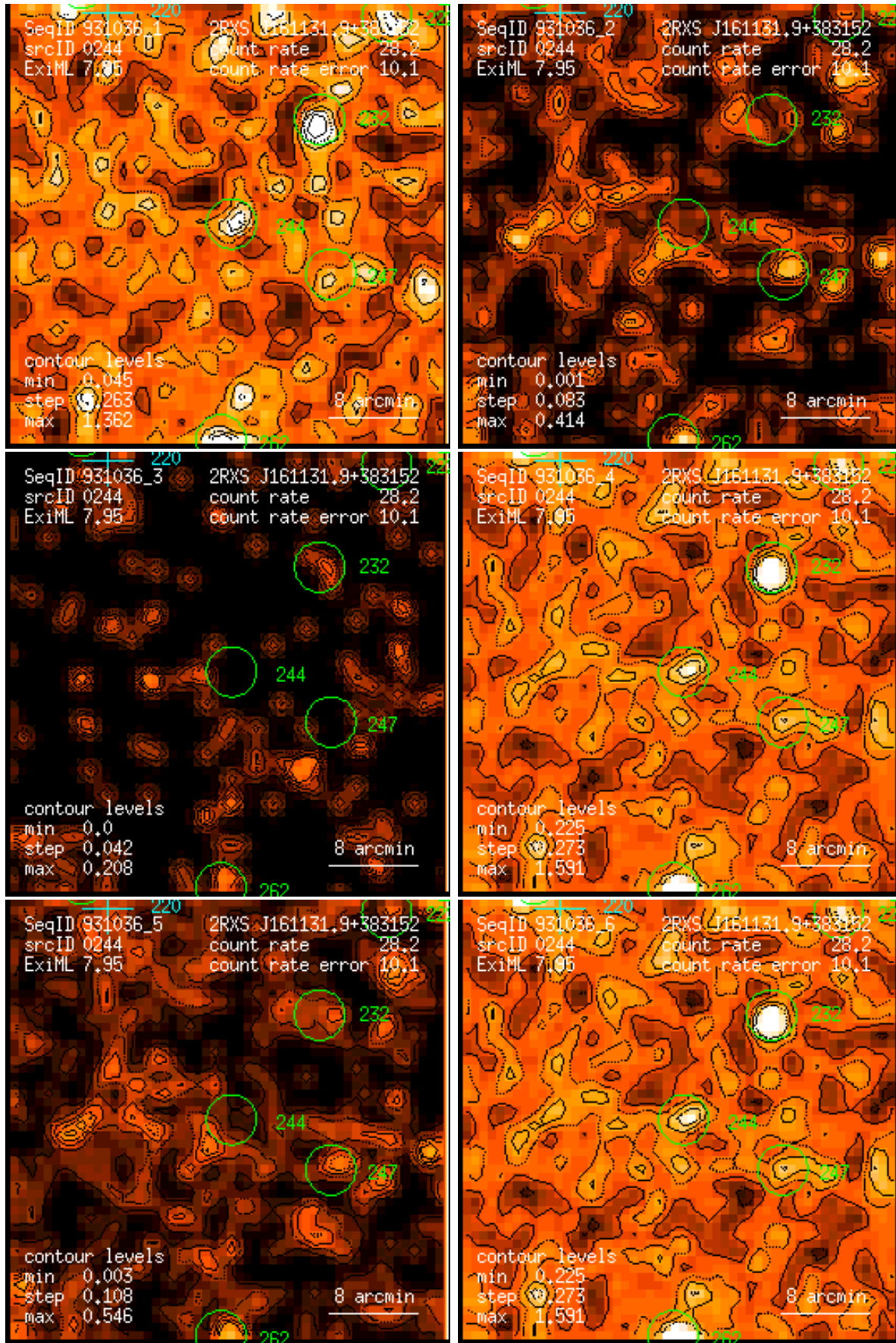
Figure 244: RASS 931036: detection 0244: band rate images, Gaussian filter: (1) PSPC channels 11 – 41, (2) 52 – 90, (3) 91 – 201, (4) 11 – 235, (5) 52 – 201, (6) 11 – 201. Broad band rates in counts/ks. Band rate contour levels in counts/ks/arcmin 2 .
