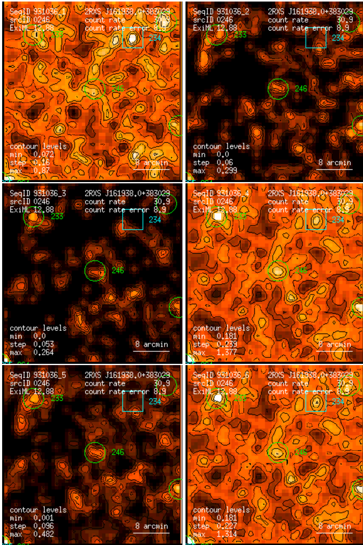
Figure 246: RASS 931036: detection 0246: band rate images, Gaussian filter: (1) PSPC channels 11 – 41, (2) 52 – 90, (3) 91 – 201, (4) 11 – 235, (5) 52 – 201, (6) 11 – 201. Broad band rates in counts/ks. Band rate contour levels in counts/ks/arcmin 2 .
