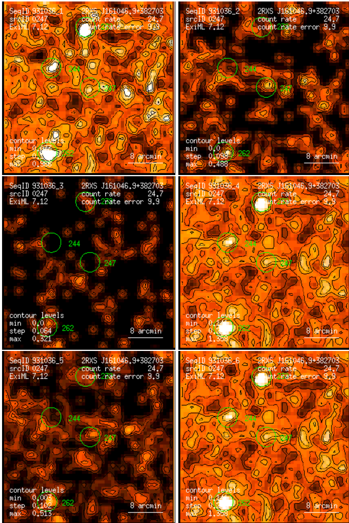
Figure 247: RASS 931036: detection 0247: band rate images, Gaussian filter: (1) PSPC channels 11 – 41, (2) 52 – 90, (3) 91 – 201, (4) 11 – 235, (5) 52 – 201, (6) 11 – 201. Broad band rates in counts/ks. Band rate contour levels in counts/ks/arcmin 2 .
