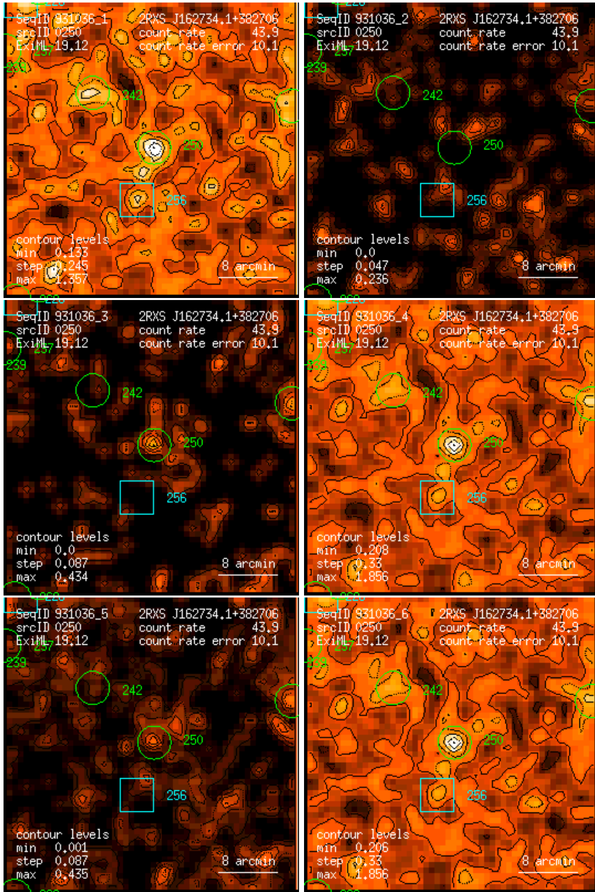
Figure 250: RASS 931036: detection 0250: band rate images, Gaussian filter: (1) PSPC channels 11 – 41, (2) 52 – 90, (3) 91 – 201, (4) 11 – 235, (5) 52 – 201, (6) 11 – 201. Broad band rates in counts/ks. Band rate contour levels in counts/ks/arcmin 2 .
