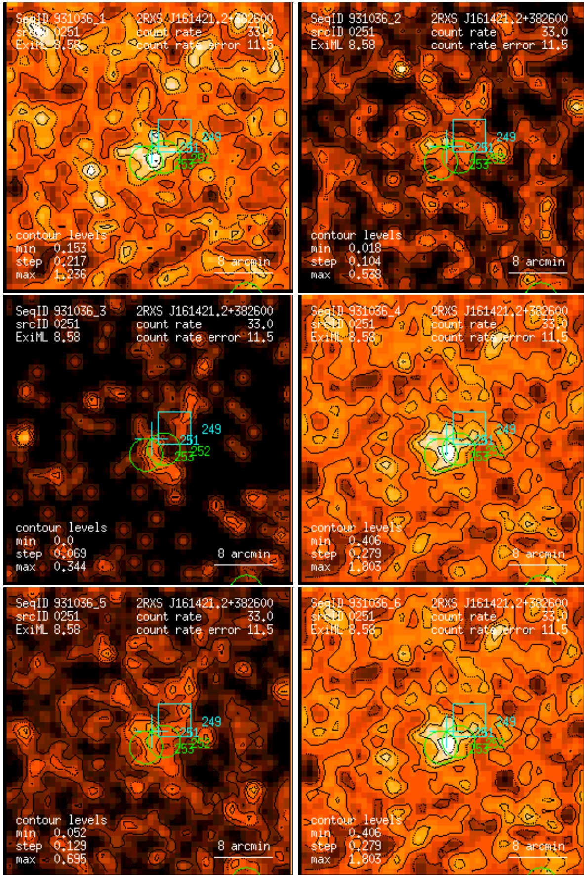
Figure 251: RASS 931036: detection 0251: band rate images, Gaussian filter: (1) PSPC channels 11 – 41, (2) 52 – 90, (3) 91 – 201, (4) 11 – 235, (5) 52 – 201, (6) 11 – 201. Broad band rates in counts/ks. Band rate contour levels in counts/ks/arcmin 2 .
