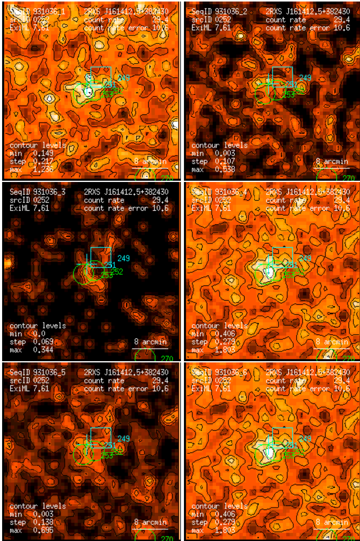
Figure 252: RASS 931036: detection 0252: band rate images, Gaussian filter: (1) PSPC channels 11 – 41, (2) 52 – 90, (3) 91 – 201, (4) 11 – 235, (5) 52 – 201, (6) 11 – 201. Broad band rates in counts/ks. Band rate contour levels in counts/ks/arcmin 2 .
