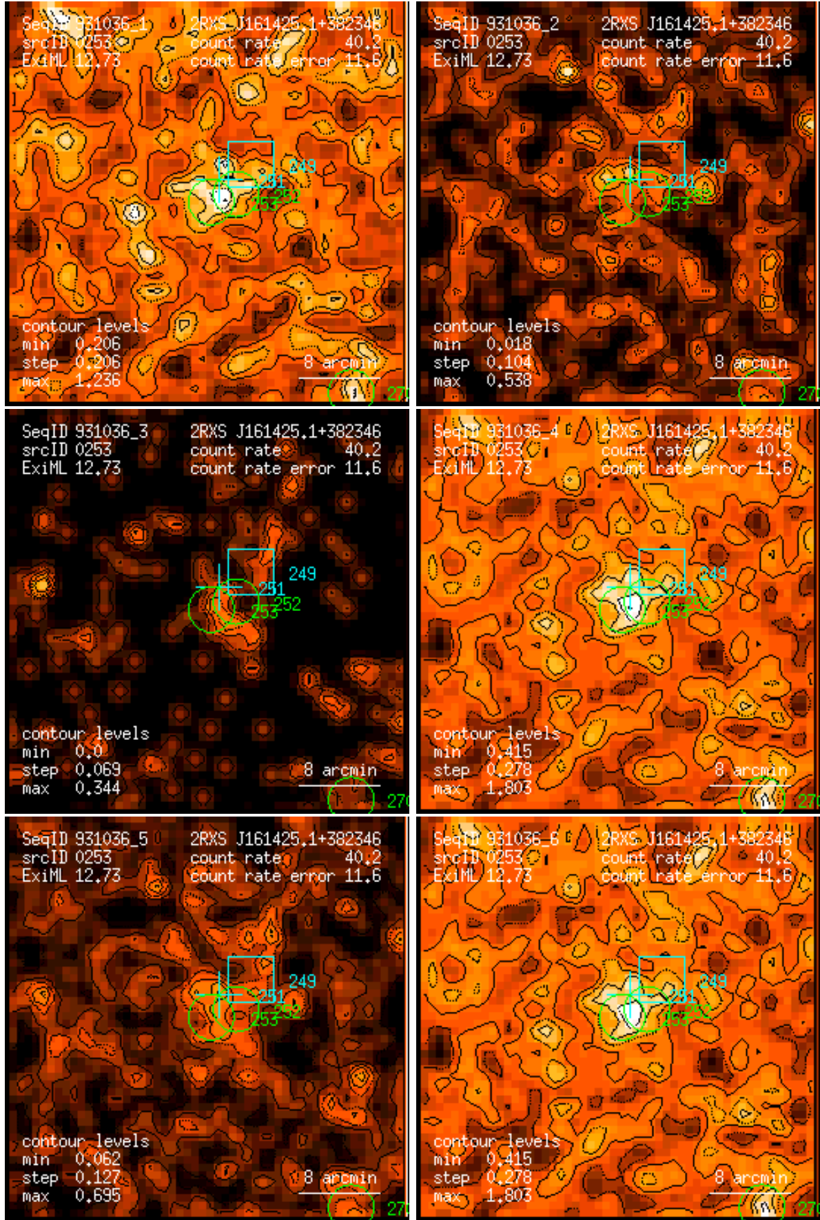
Figure 253: RASS 931036: detection 0253: band rate images, Gaussian filter: (1) PSPC channels 11 – 41, (2) 52 – 90, (3) 91 – 201, (4) 11 – 235, (5) 52 – 201, (6) 11 – 201. Broad band rates in counts/ks. Band rate contour levels in counts/ks/arcmin 2 .
