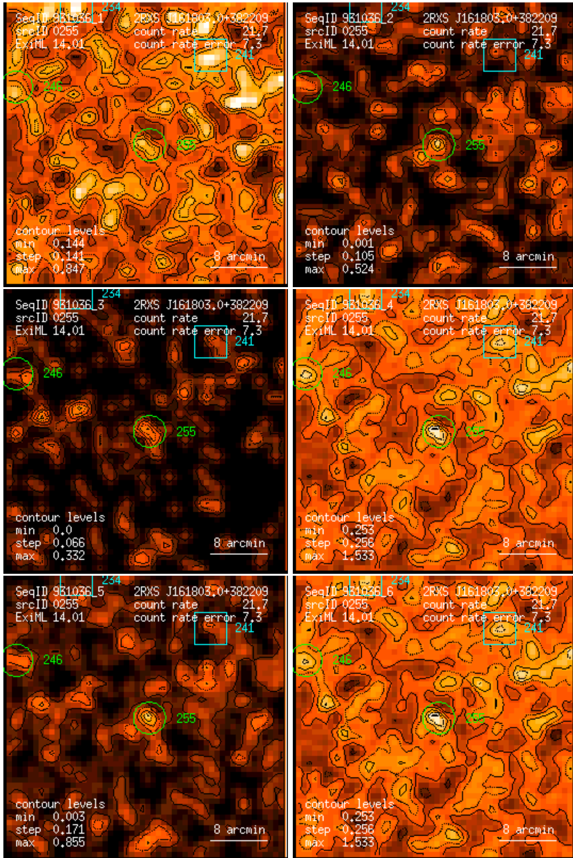
Figure 255: RASS 931036: detection 0255: band rate images, Gaussian filter: (1) PSPC channels 11 – 41, (2) 52 – 90, (3) 91 – 201, (4) 11 – 235, (5) 52 – 201, (6) 11 – 201. Broad band rates in counts/ks. Band rate contour levels in counts/ks/arcmin 2 .
