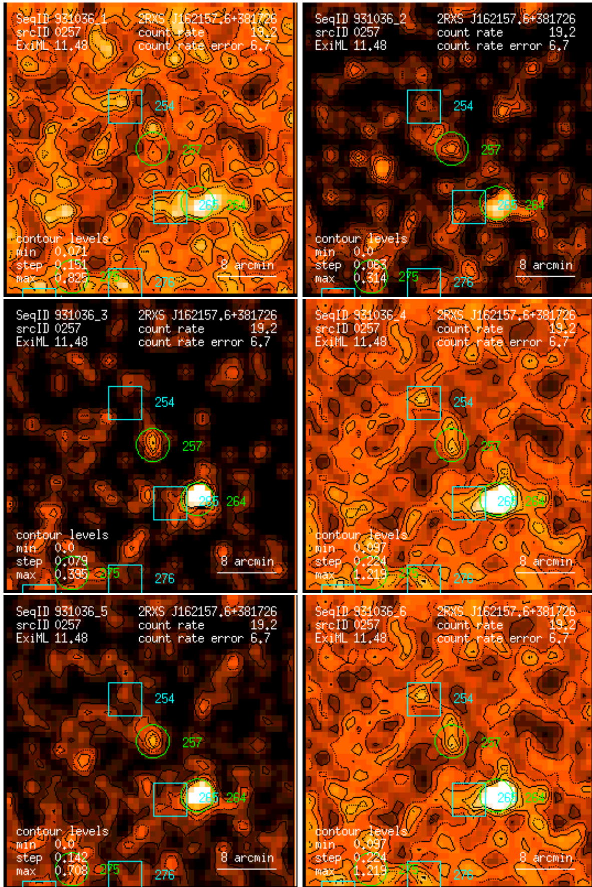
Figure 257: RASS 931036: detection 0257: band rate images, Gaussian filter: (1) PSPC channels 11 – 41, (2) 52 – 90, (3) 91 – 201, (4) 11 – 235, (5) 52 – 201, (6) 11 – 201. Broad band rates in counts/ks. Band rate contour levels in counts/ks/arcmin 2 .
