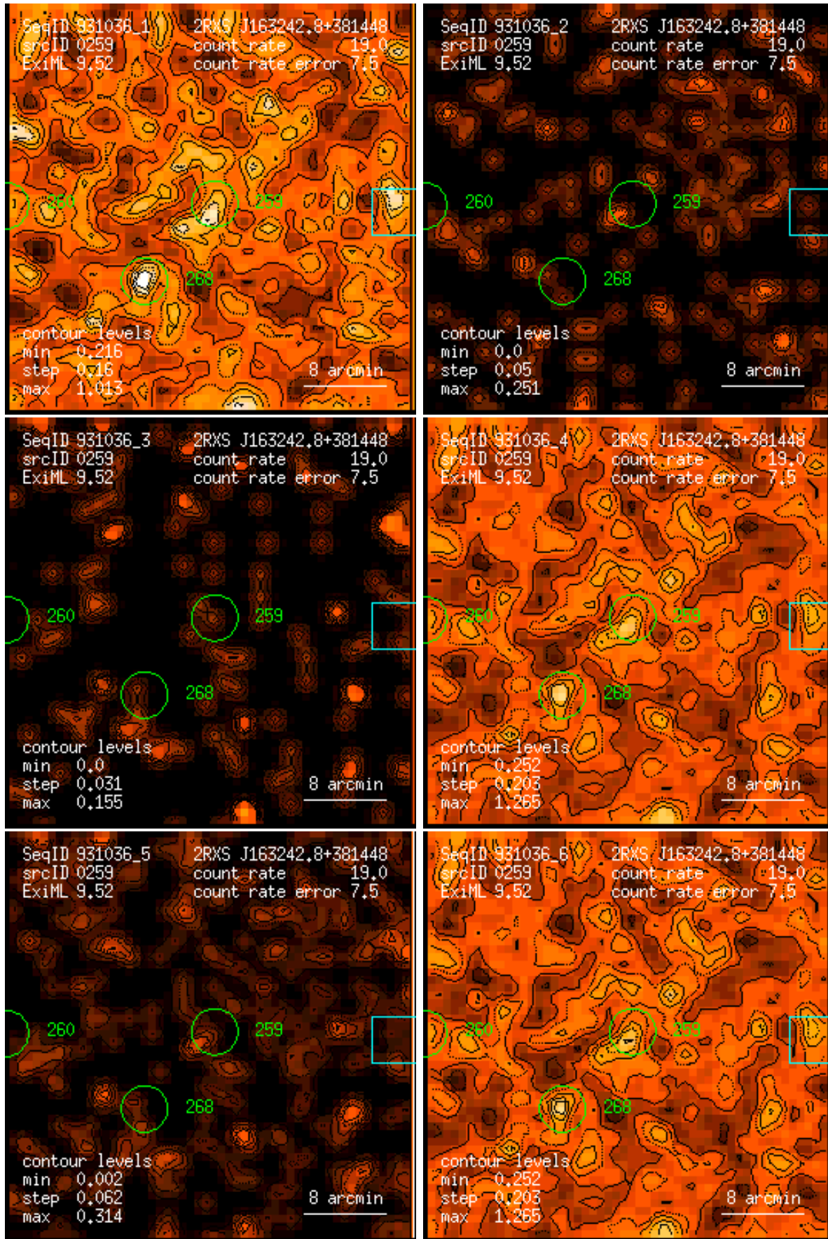
Figure 259: RASS 931036: detection 0259: band rate images, Gaussian filter: (1) PSPC channels 11 – 41, (2) 52 – 90, (3) 91 – 201, (4) 11 – 235, (5) 52 – 201, (6) 11 – 201. Broad band rates in counts/ks. Band rate contour levels in counts/ks/arcmin 2 .
