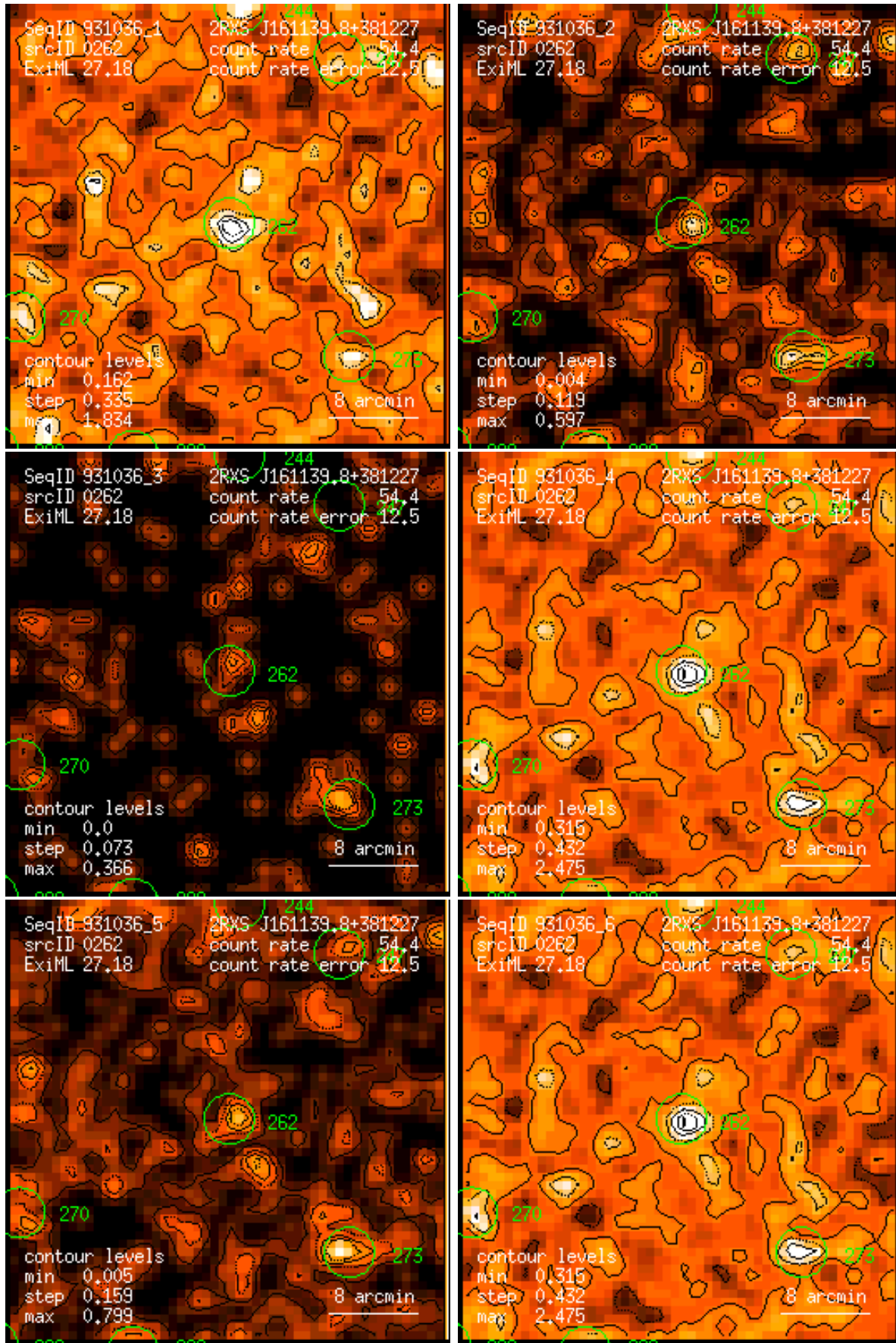
Figure 262: RASS 931036: detection 0262: band rate images, Gaussian filter: (1) PSPC channels 11 – 41, (2) 52 – 90, (3) 91 – 201, (4) 11 – 235, (5) 52 – 201, (6) 11 – 201. Broad band rates in counts/ks. Band rate contour levels in counts/ks/arcmin 2 .
