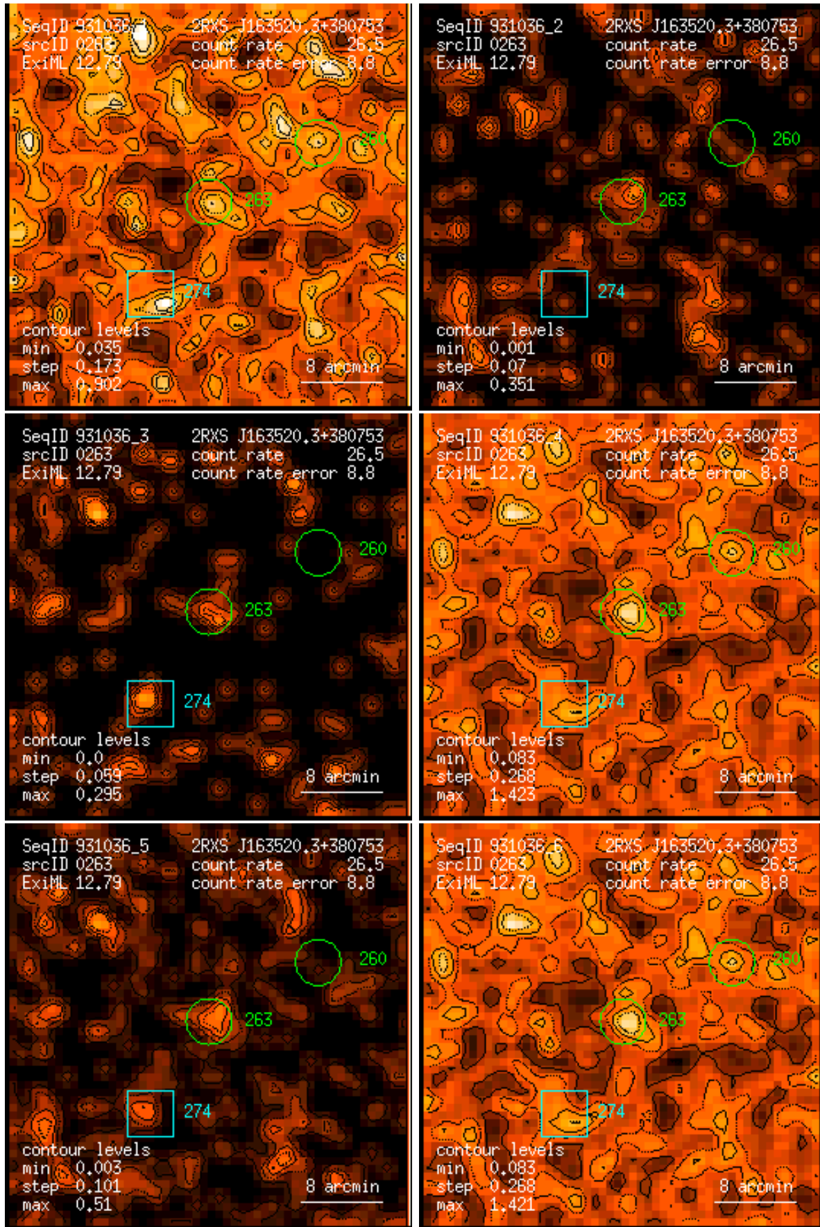
Figure 263: RASS 931036: detection 0263: band rate images, Gaussian filter: (1) PSPC channels 11 – 41, (2) 52 – 90, (3) 91 – 201, (4) 11 – 235, (5) 52 – 201, (6) 11 – 201. Broad band rates in counts/ks. Band rate contour levels in counts/ks/arcmin 2 .
