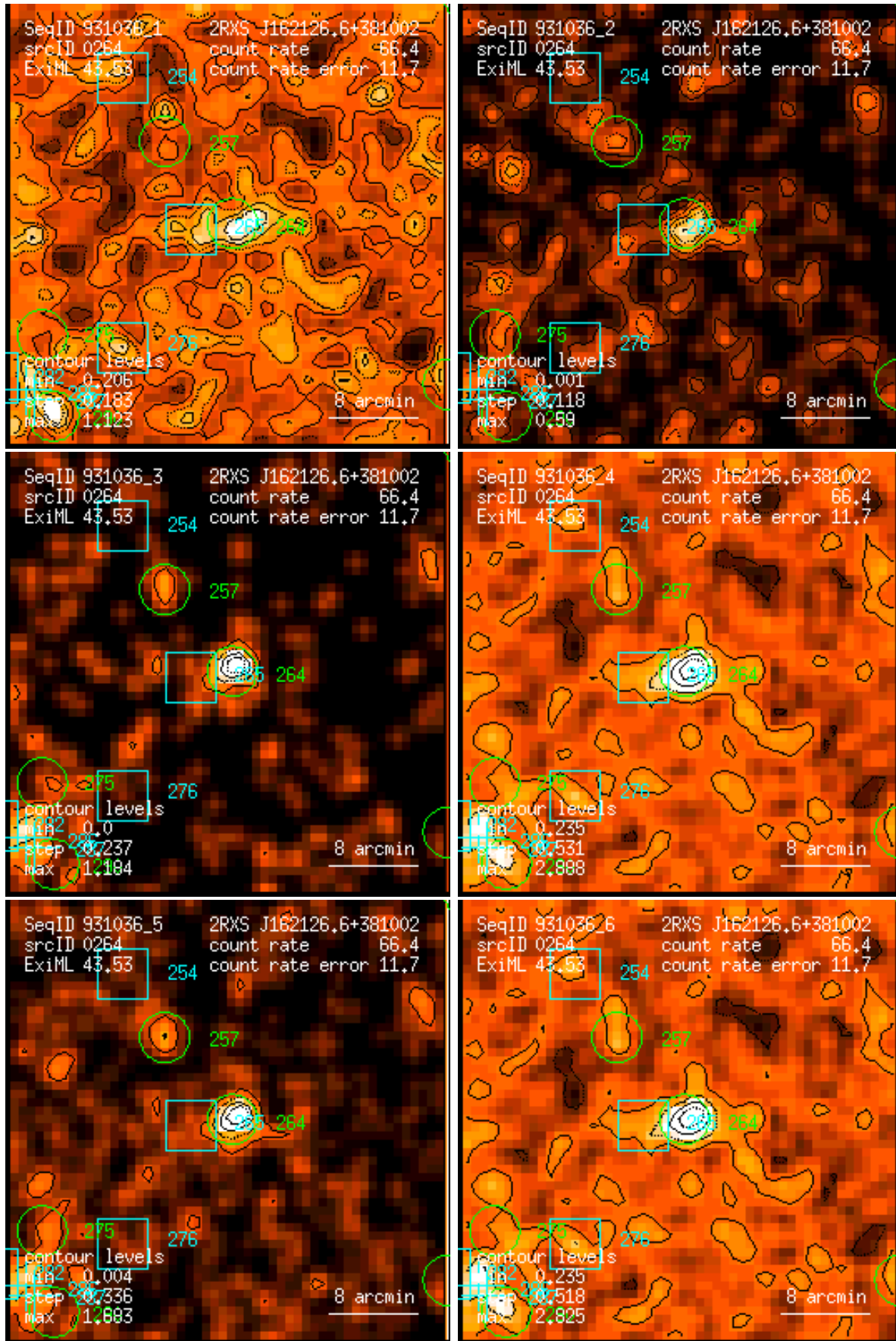
Figure 264: RASS 931036: detection 0264: band rate images, Gaussian filter: (1) PSPC channels 11 – 41, (2) 52 – 90, (3) 91 – 201, (4) 11 – 235, (5) 52 – 201, (6) 11 – 201. Broad band rates in counts/ks. Band rate contour levels in counts/ks/arcmin 2 .
