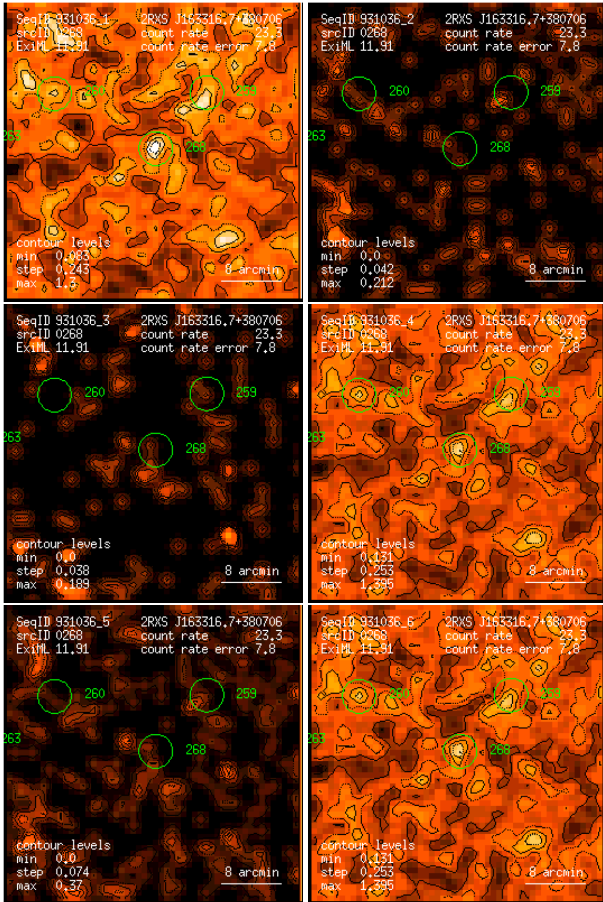
Figure 268: RASS 931036: detection 0268: band rate images, Gaussian filter: (1) PSPC channels 11 – 41, (2) 52 – 90, (3) 91 – 201, (4) 11 – 235, (5) 52 – 201, (6) 11 – 201. Broad band rates in counts/ks. Band rate contour levels in counts/ks/arcmin 2 .
