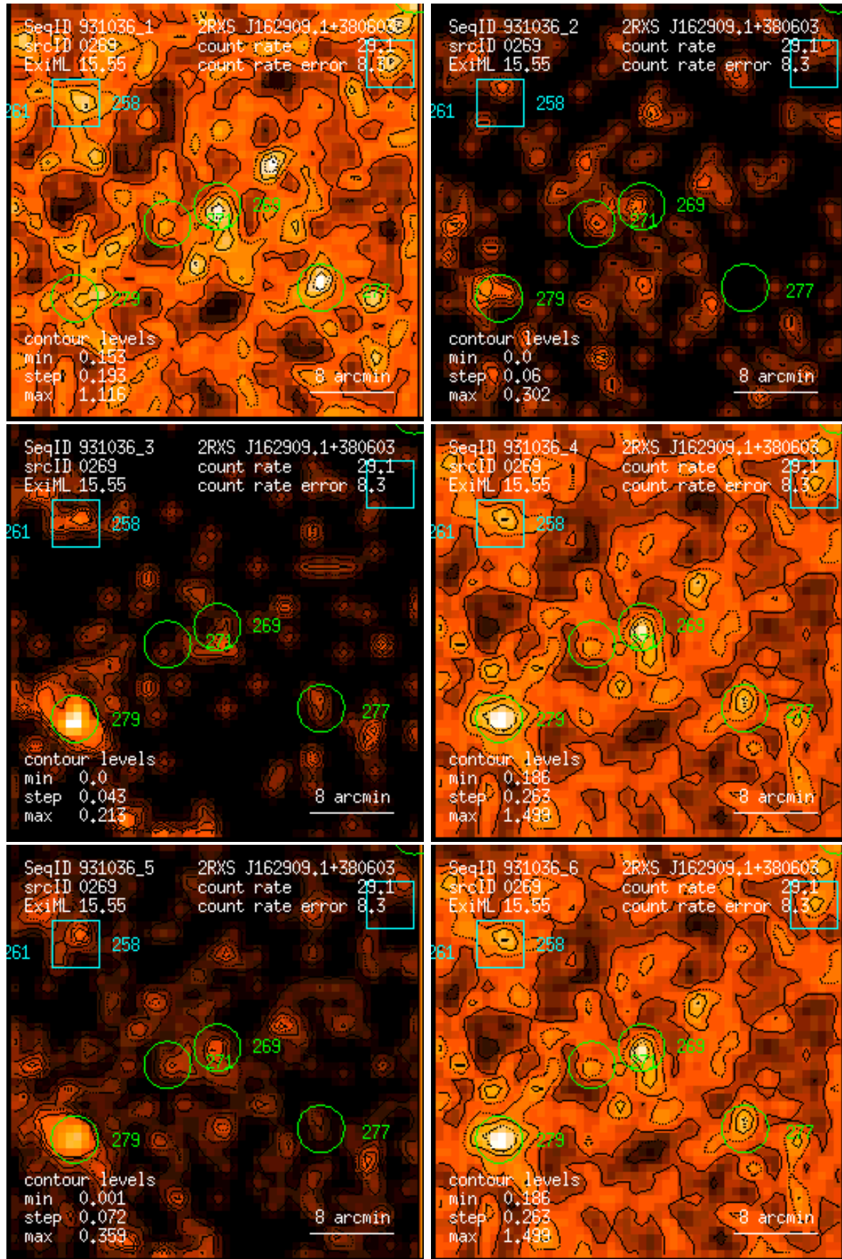
Figure 269: RASS 931036: detection 0269: band rate images, Gaussian filter: (1) PSPC channels 11 – 41, (2) 52 – 90, (3) 91 – 201, (4) 11 – 235, (5) 52 – 201, (6) 11 – 201. Broad band rates in counts/ks. Band rate contour levels in counts/ks/arcmin 2 .
