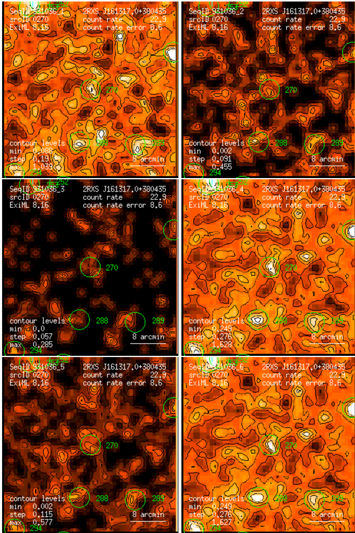
Figure 270: RASS 931036: detection 0270: band rate images, Gaussian filter: (1) PSPC channels 11 – 41, (2) 52 – 90, (3) 91 – 201, (4) 11 – 235, (5) 52 – 201, (6) 11 – 201. Broad band rates in counts/ks. Band rate contour levels in counts/ks/arcmin 2 .
