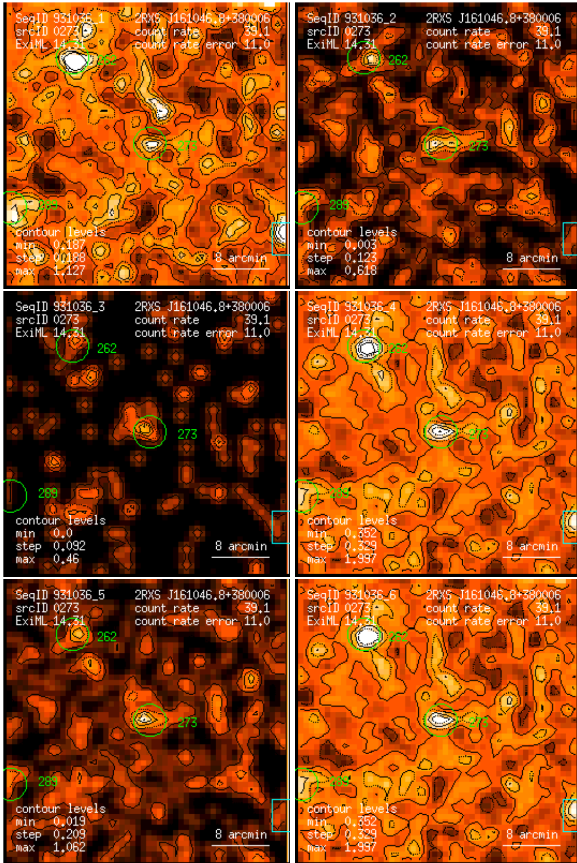
Figure 273: RASS 931036: detection 0273: band rate images, Gaussian filter: (1) PSPC channels 11 – 41, (2) 52 – 90, (3) 91 – 201, (4) 11 – 235, (5) 52 – 201, (6) 11 – 201. Broad band rates in counts/ks. Band rate contour levels in counts/ks/arcmin 2 .
