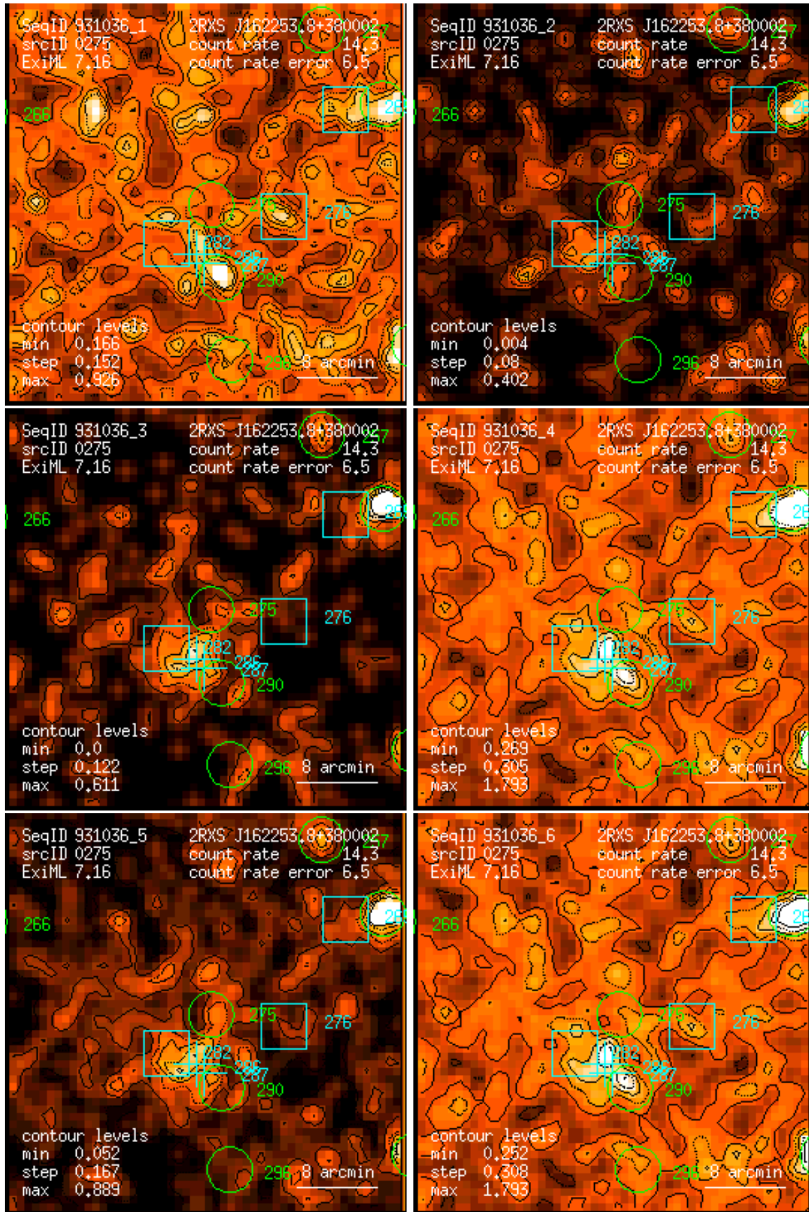
Figure 275: RASS 931036: detection 0275: band rate images, Gaussian filter: (1) PSPC channels 11 – 41, (2) 52 – 90, (3) 91 – 201, (4) 11 – 235, (5) 52 – 201, (6) 11 – 201. Broad band rates in counts/ks. Band rate contour levels in counts/ks/arcmin 2 .
